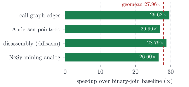
Figure 4: WCOJ vs. binary-join speedup on the four key-generation variants of the triangle fixture ( 3 \times 65,536 input rows, \approx 4.19\text{M} output triples). Single-system ablation; the dashed line is the geometric mean.
