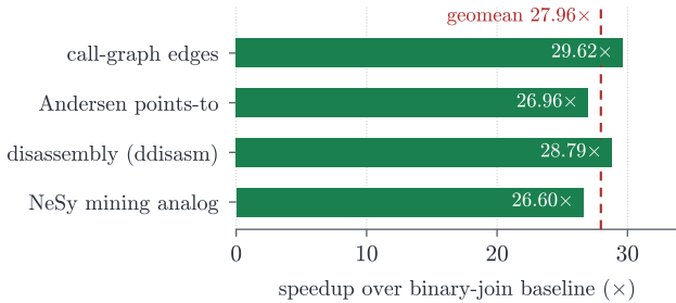
Figure 4: WCOJ vs. binary-join speedup on the four key-generation variants of the triangle fixture (Table 8). Single-system ablation; the dashed line is the geometric mean.
