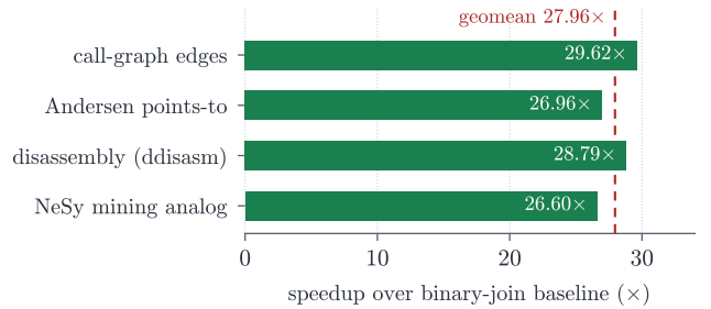
Figure 4: WCOJ vs. binary-join speedup on the four key-generation variants of the triangle fixture ( 3 \times 65,536 input rows, \approx 4.19\text{M} output triples). Single-system ablation; the dashed line is the geometric mean.
