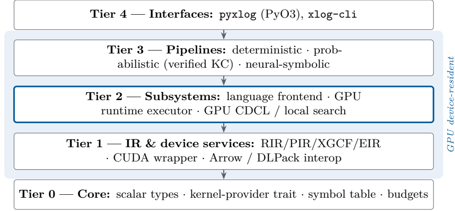
Figure 1: xlog crate hierarchy. Each tier depends only on strictly lower tiers; all runtime semantic state is device-resident, while the host handles only orchestration, I/O, and compilation.
