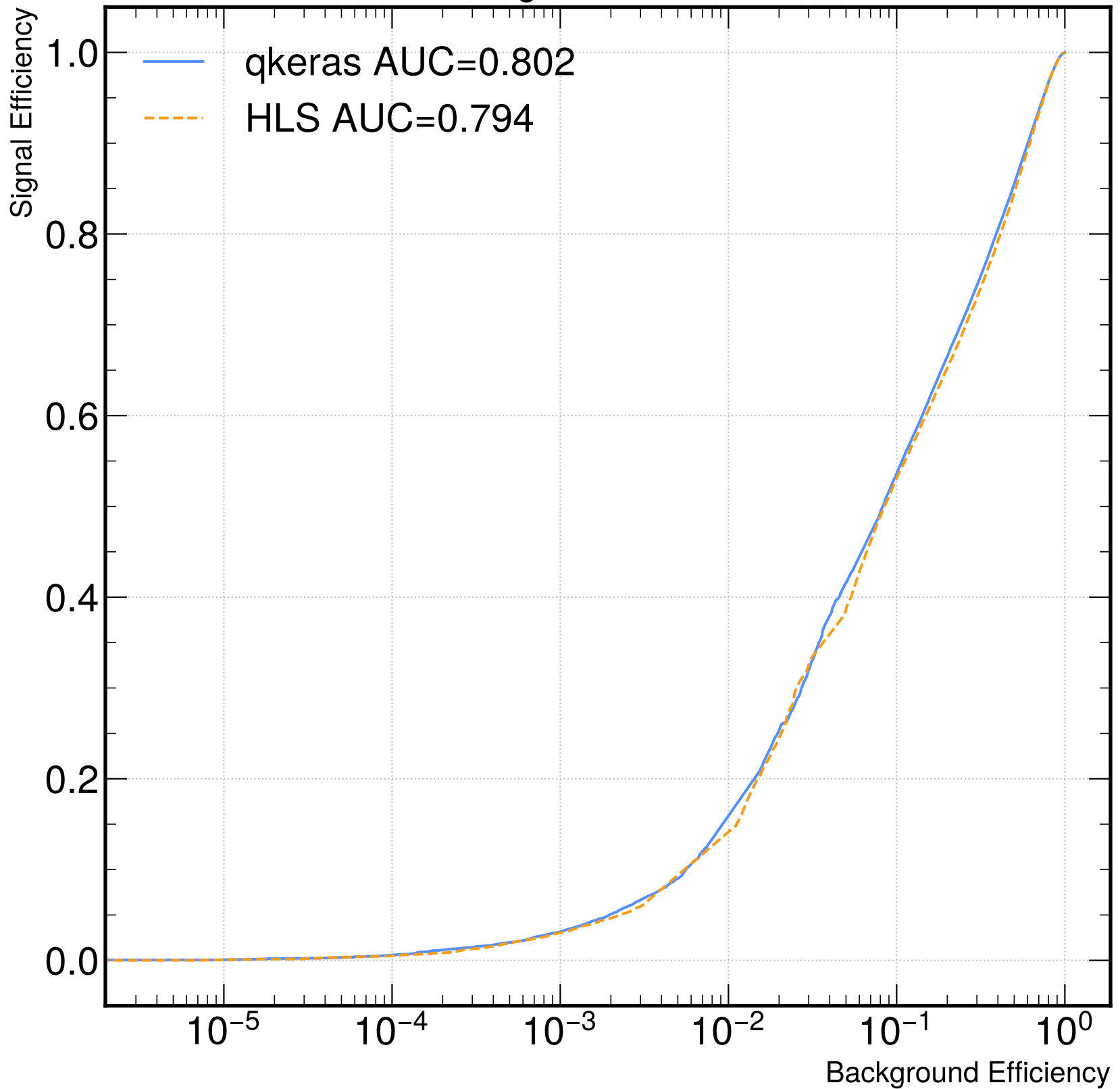
L1 LLP Tag Qk Model ROC Curve
