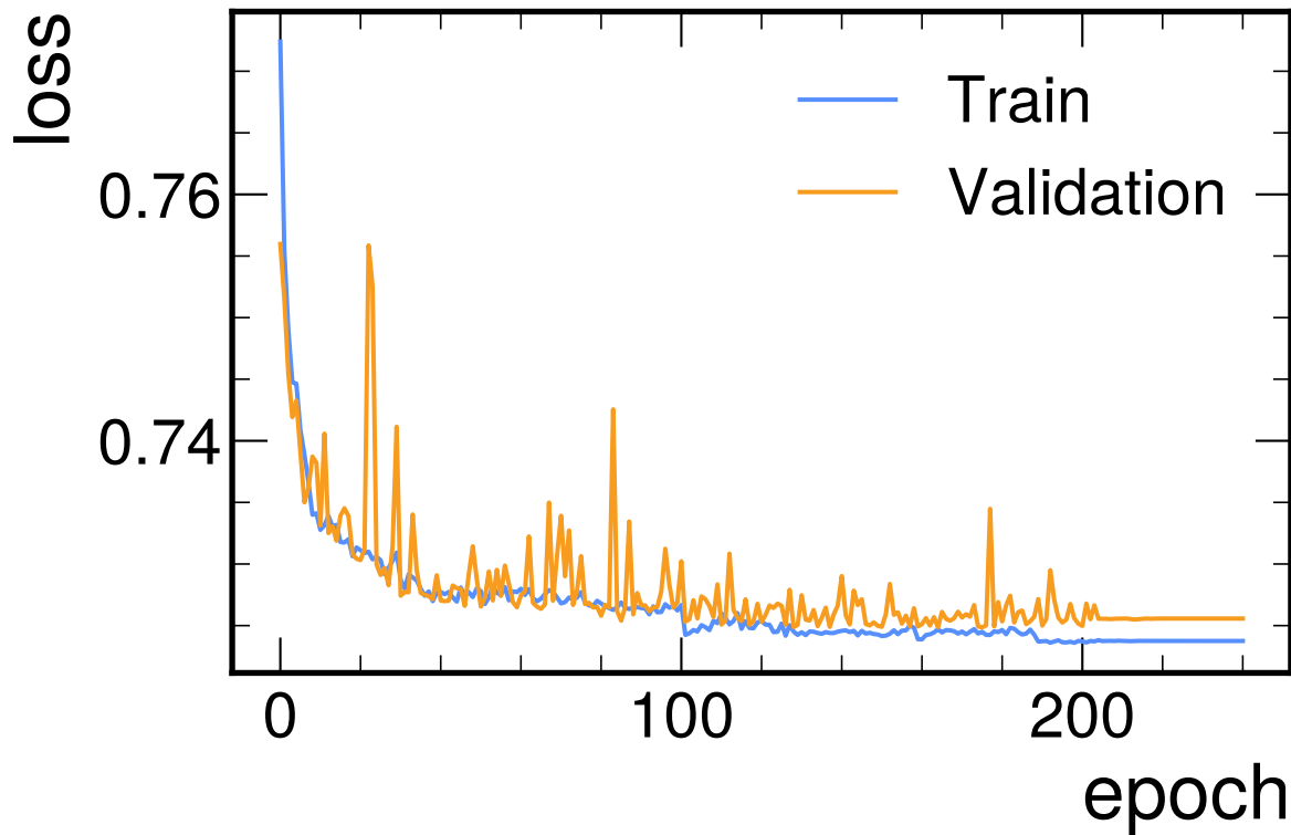
Model Loss
