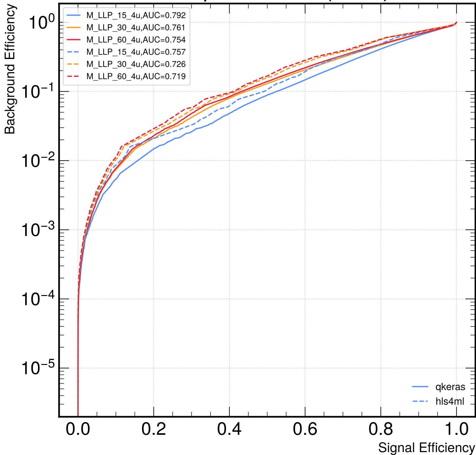
HLS vs. qkeras ROC Curves (hh--> 4u)
