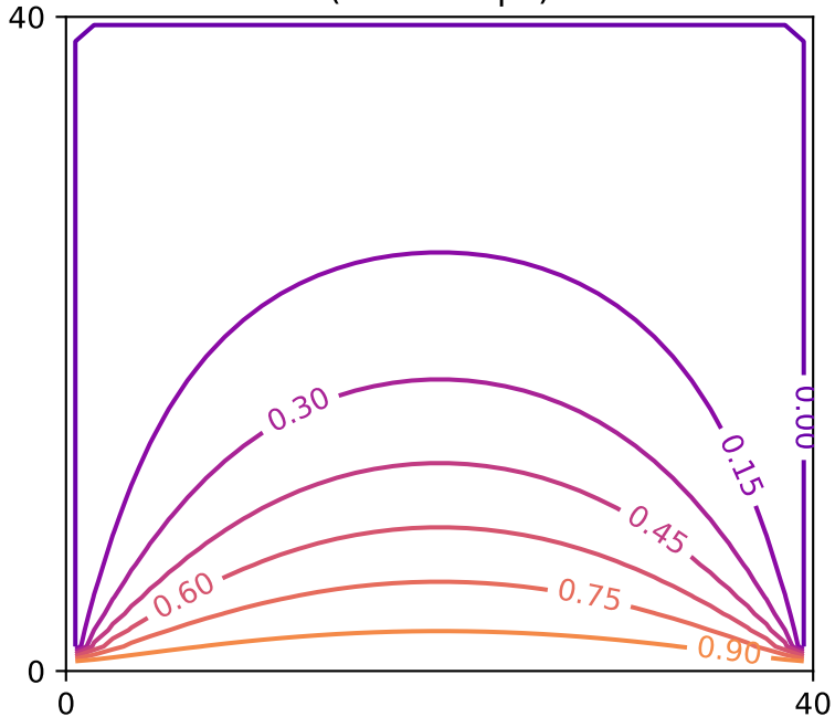
Jacobi (3629 steps)
