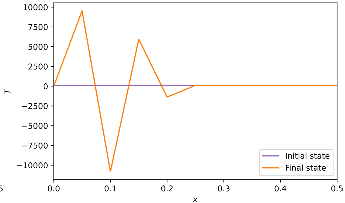
Unstable, r = 1.96
