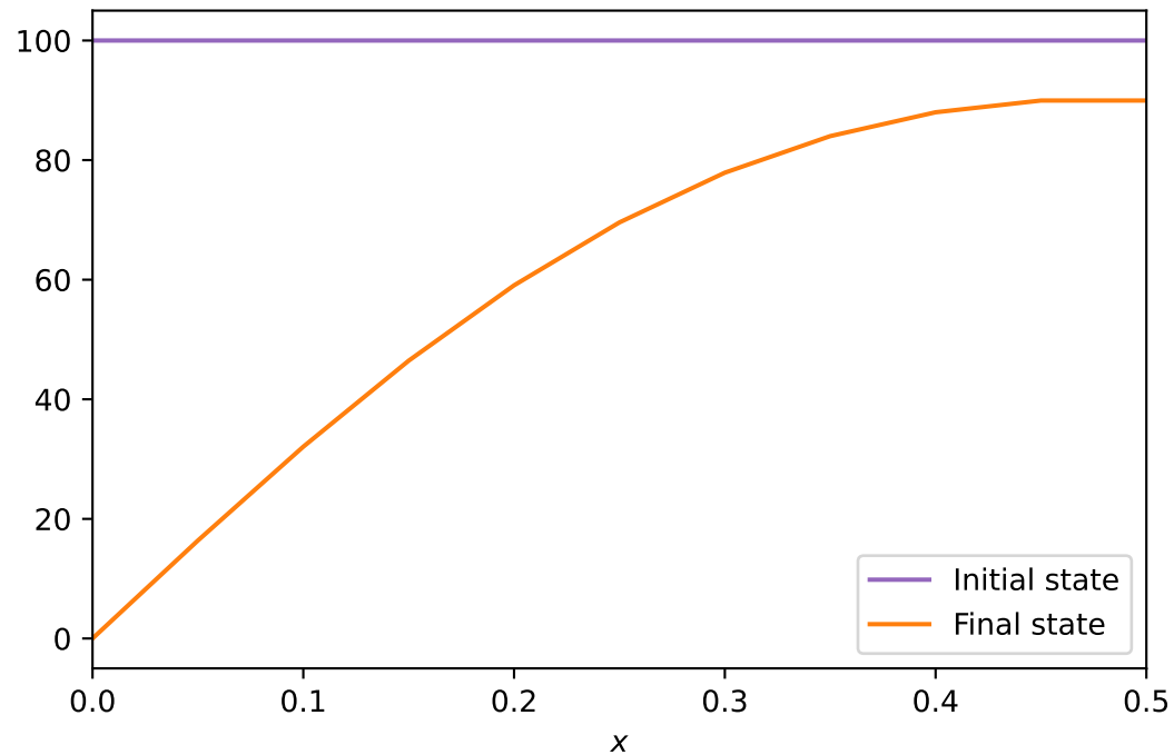
Stable, r = 0.20
