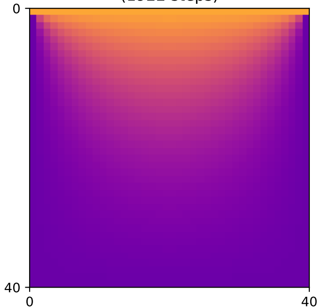
Gauss-Seidel RB (1922 steps)
