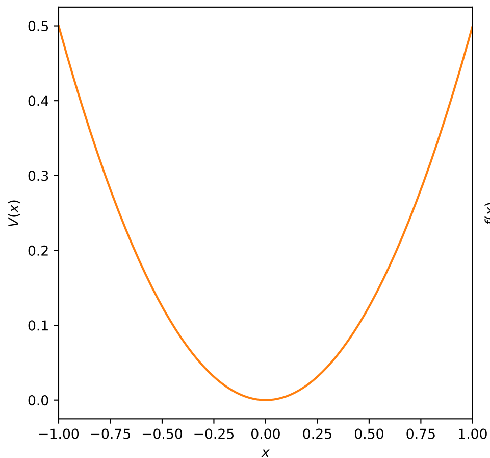
Harmonic( k = 1 )
