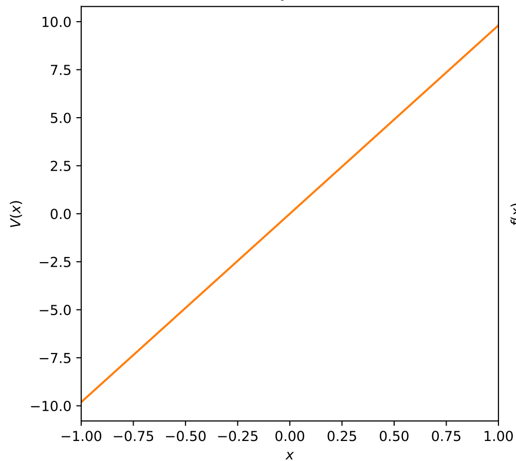
Gravity( m = 1 )
