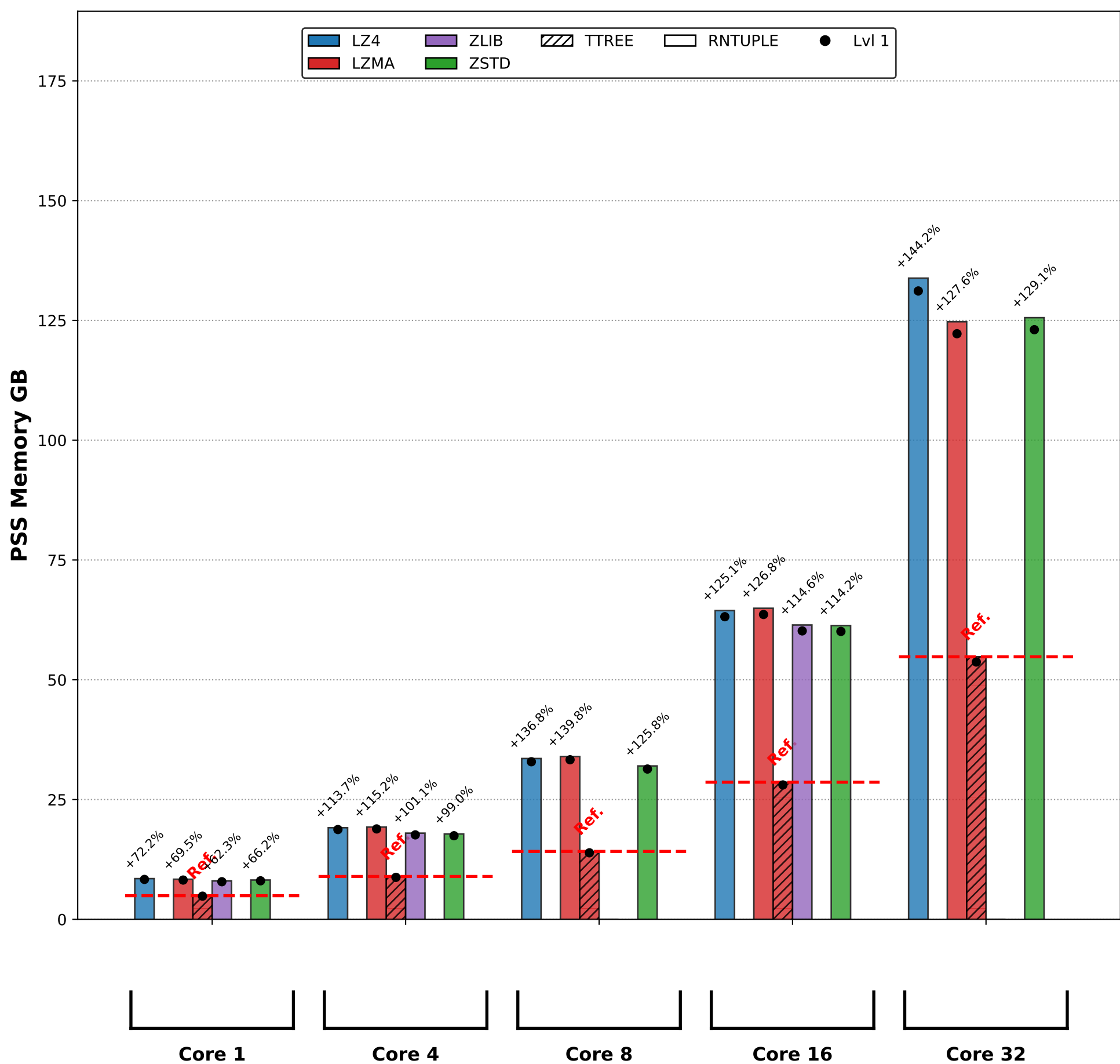
Global Analysis: PSS Memory GB
