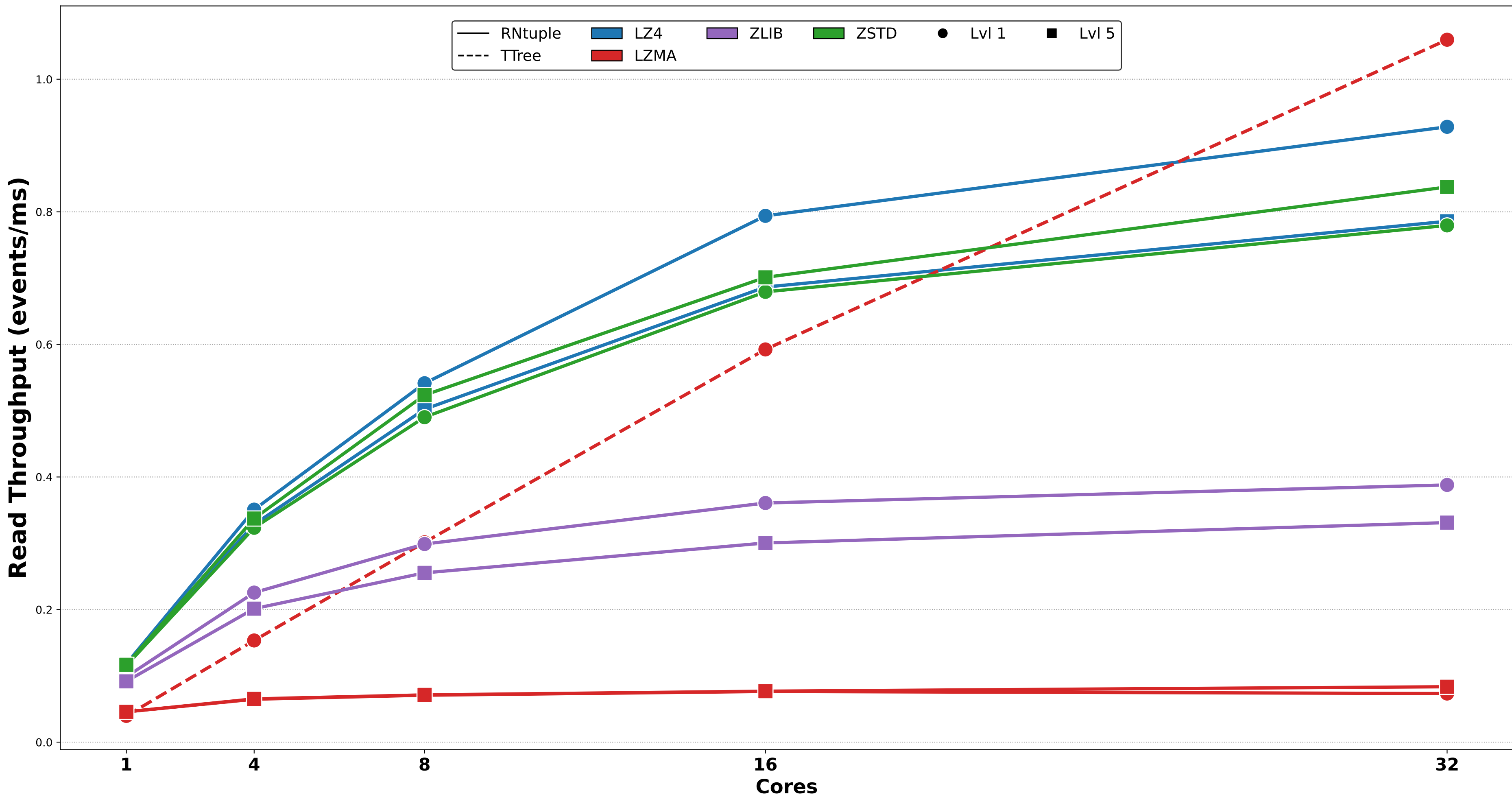
Scaling Trends: Read Throughput (events/ms)
