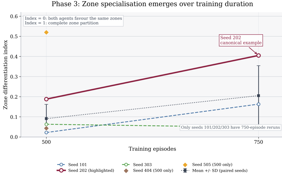
Figure 4.1: Zone differentiation growth for rainbow-lite showing dependence on training budget.
