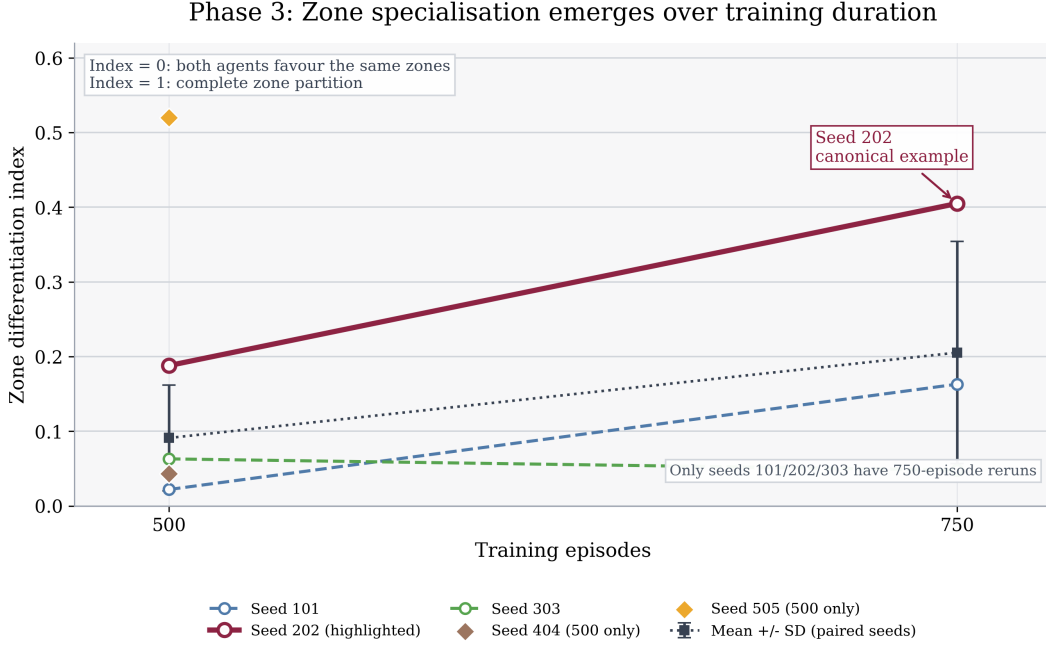
Figure 4.1: Zone differentiation growth for rainbow-lite at s2 showing dependence on training budget.
