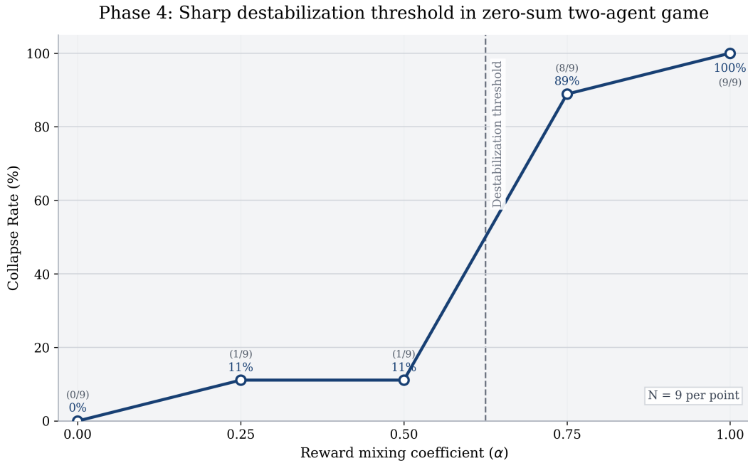
Figure 4.2: Collapse rates by \alpha in the two-agent zero-sum game.
