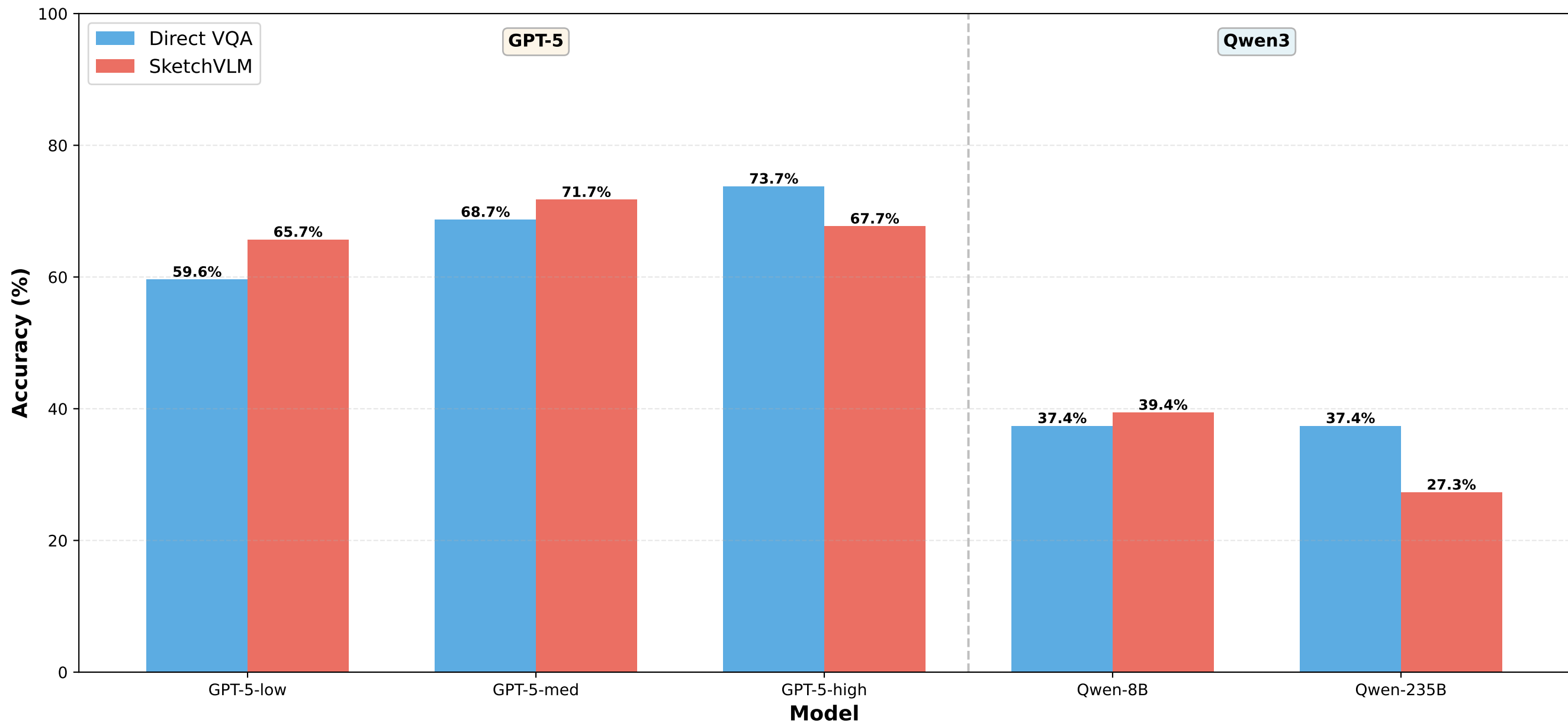
Ball Physics: Direct VQA vs SketchVLM Across All Models
