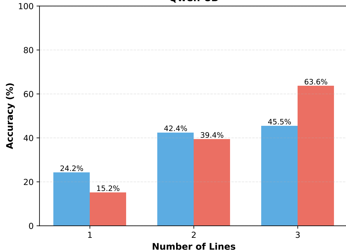
Qwen-8B
