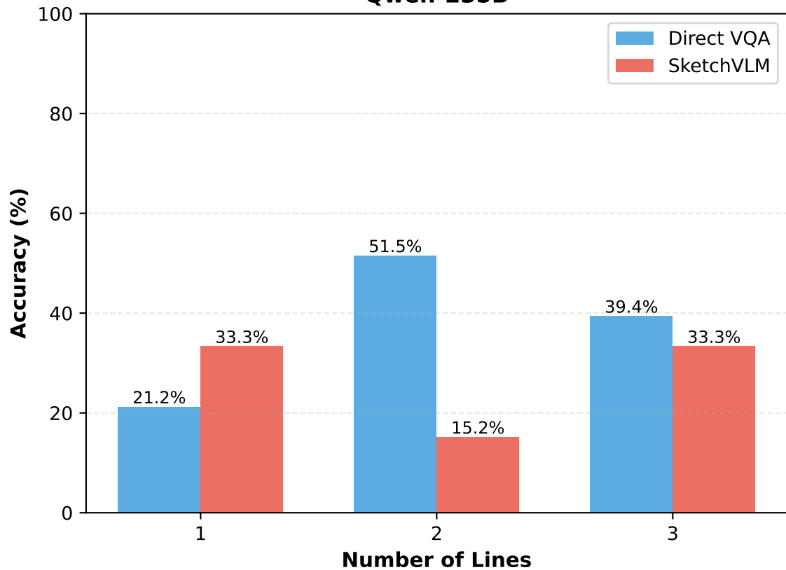
Qwen-235B
