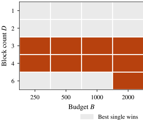
Pooled (superseded) (config. 8 wins 9/20)
