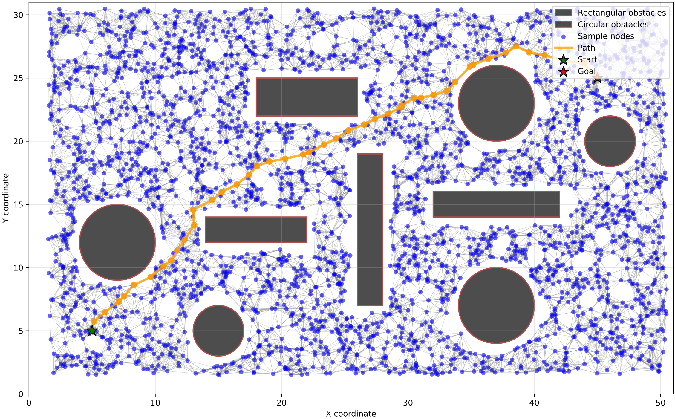
PRM Roadmap: Nodes, Edges, Obstacles, and Path
