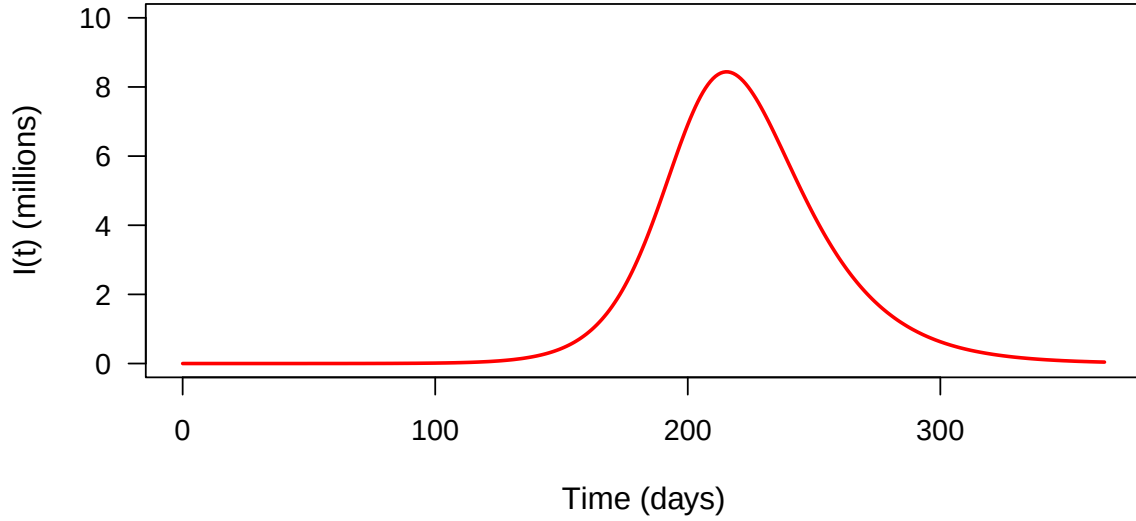
Figure 2: Number of infectives over time with parameters \beta = 2/14 infections per day, \gamma = 1/14 removals per day, N = 55,000,000 and \iota = 10 .
