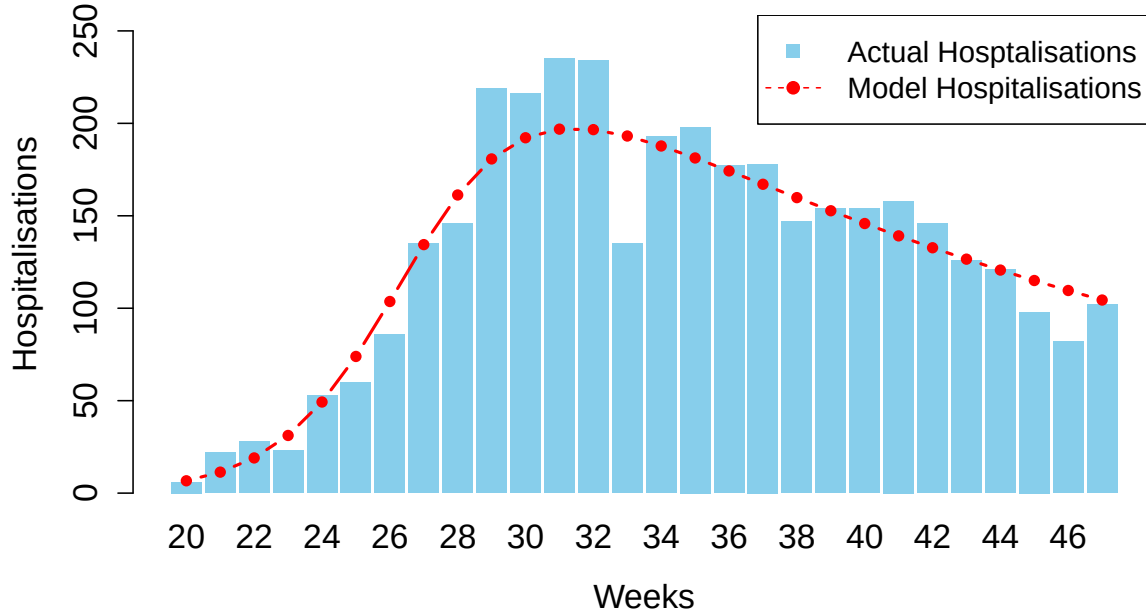
Figure 3: Fitted model predicted hospitalisations (red) and actual hospitalisations (blue) across epidemiological weeks 20 - 47 for RSV in England.
