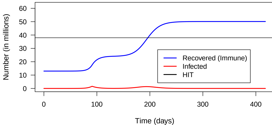
Figure 9: Proportion of immune people compared to HIT, demonstrating overshoot.
