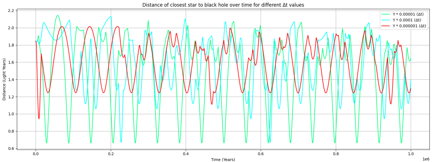
Figure 11: Distance of closest star to black hole across 1000000 years for various timesteps.
