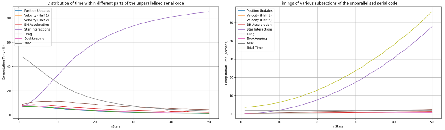
Figure 3: Distribution of time within different parts of the unparallelised serial code.
