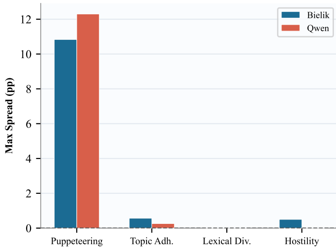
Permutation Spread (p0/p1/p2)
