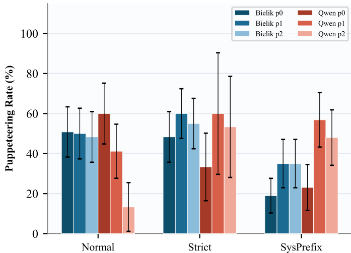
Order Effect by Prompt Condition
