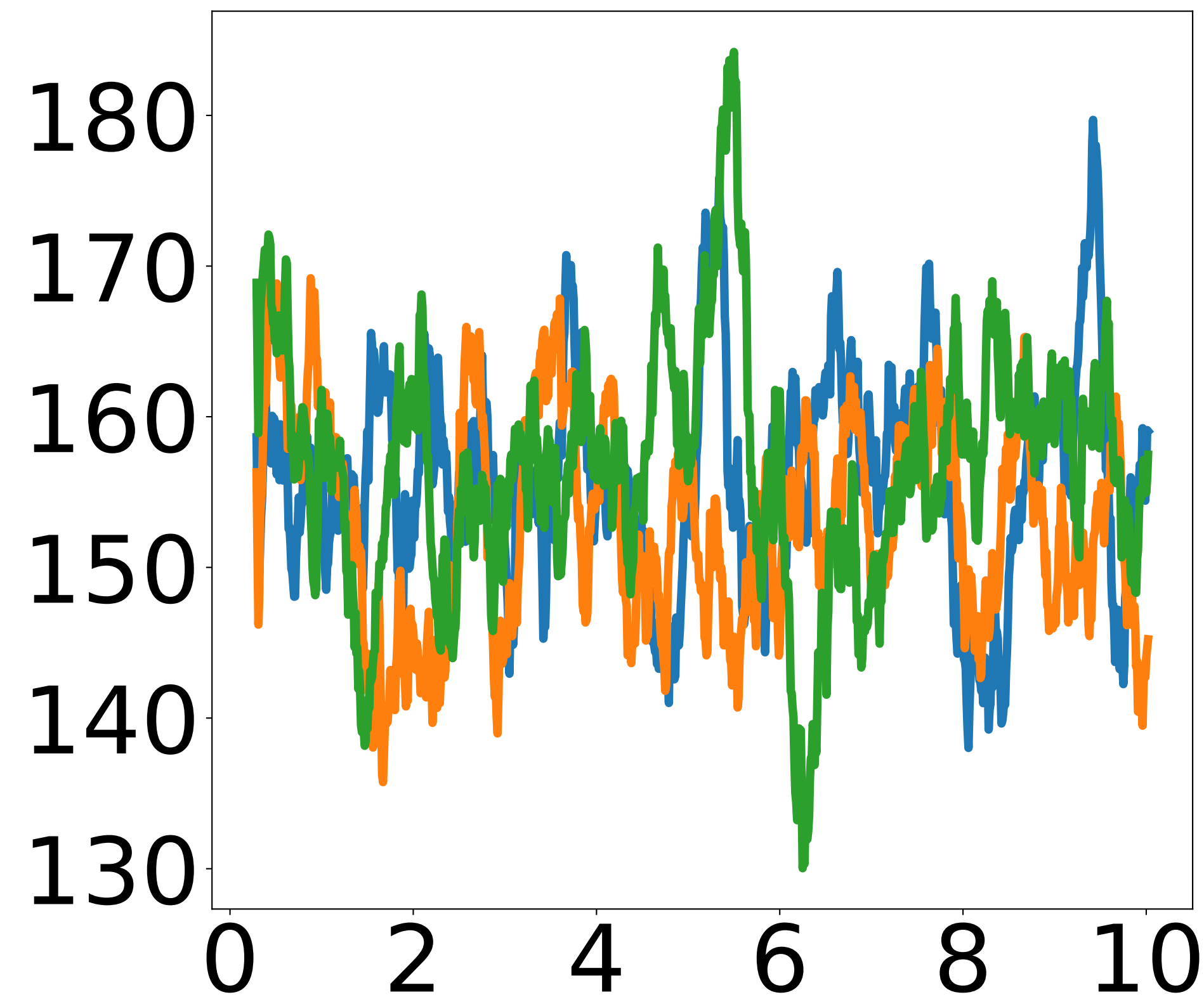
Octanethiol
