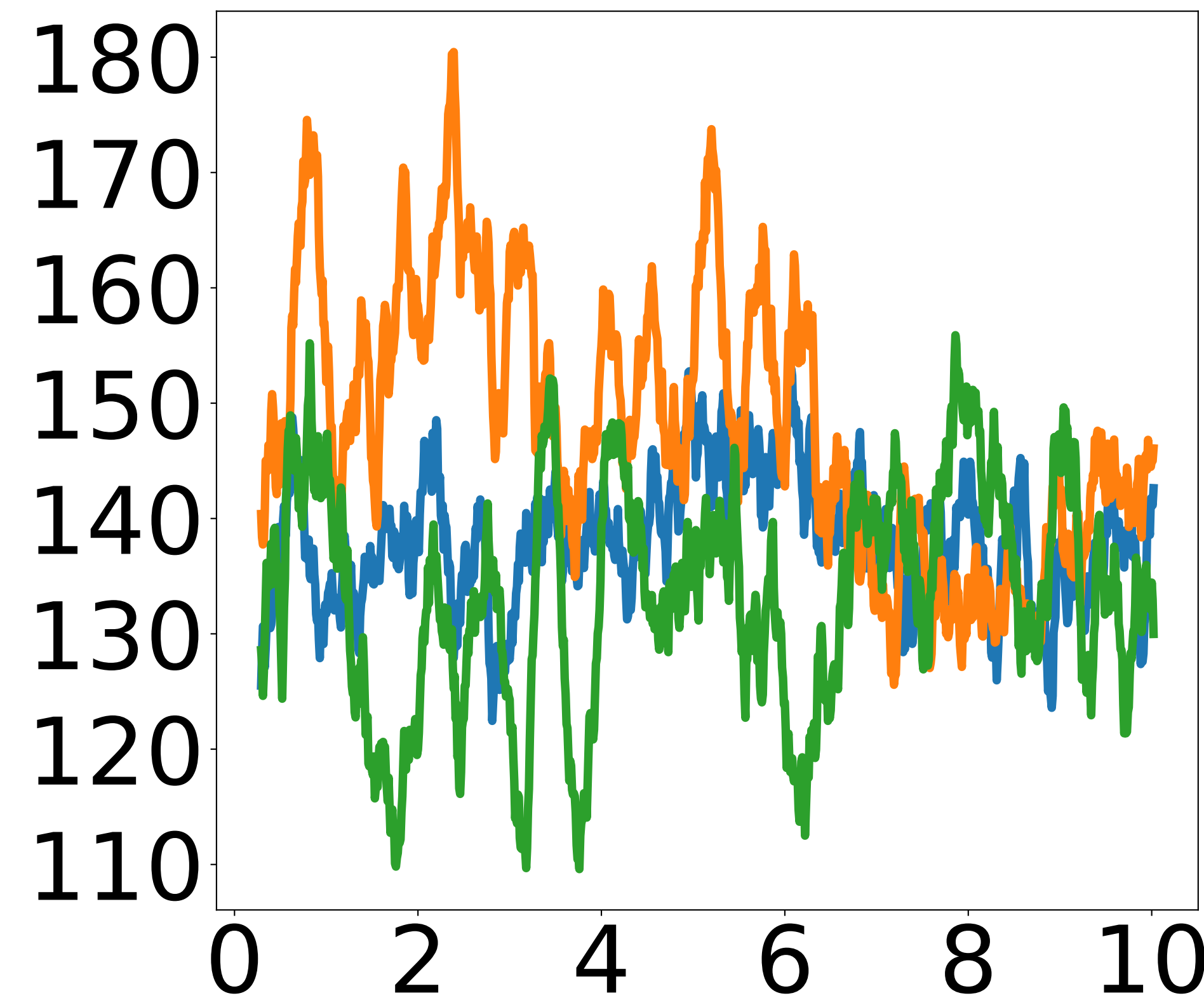
Dodecanethiol
