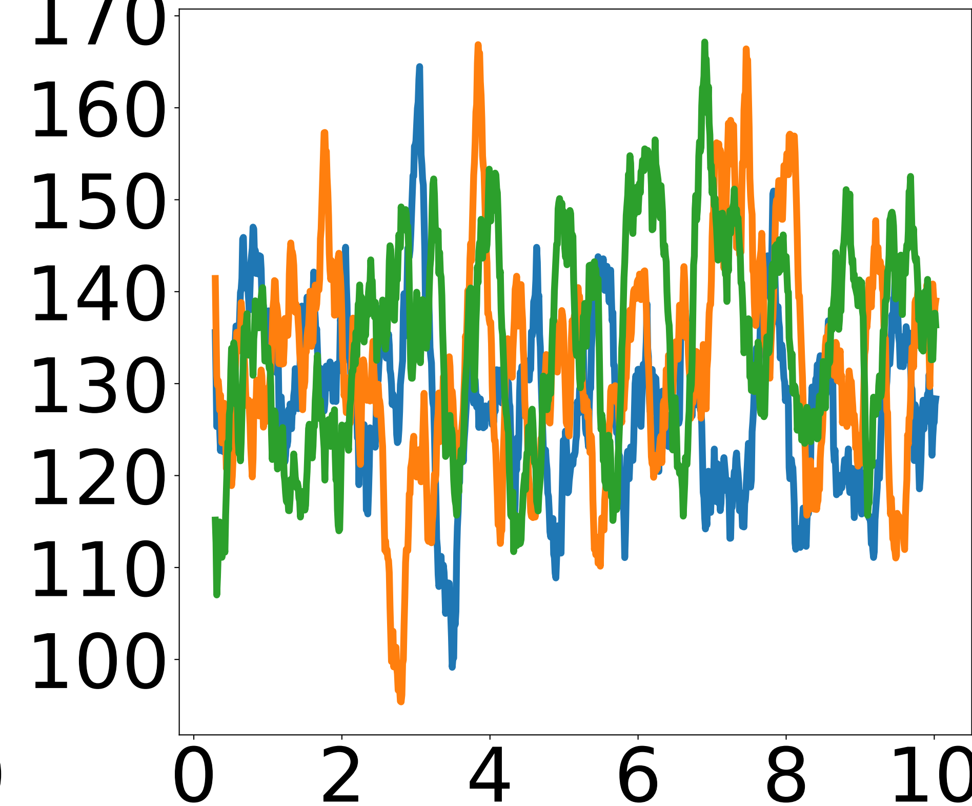
Hexadecanethiol
