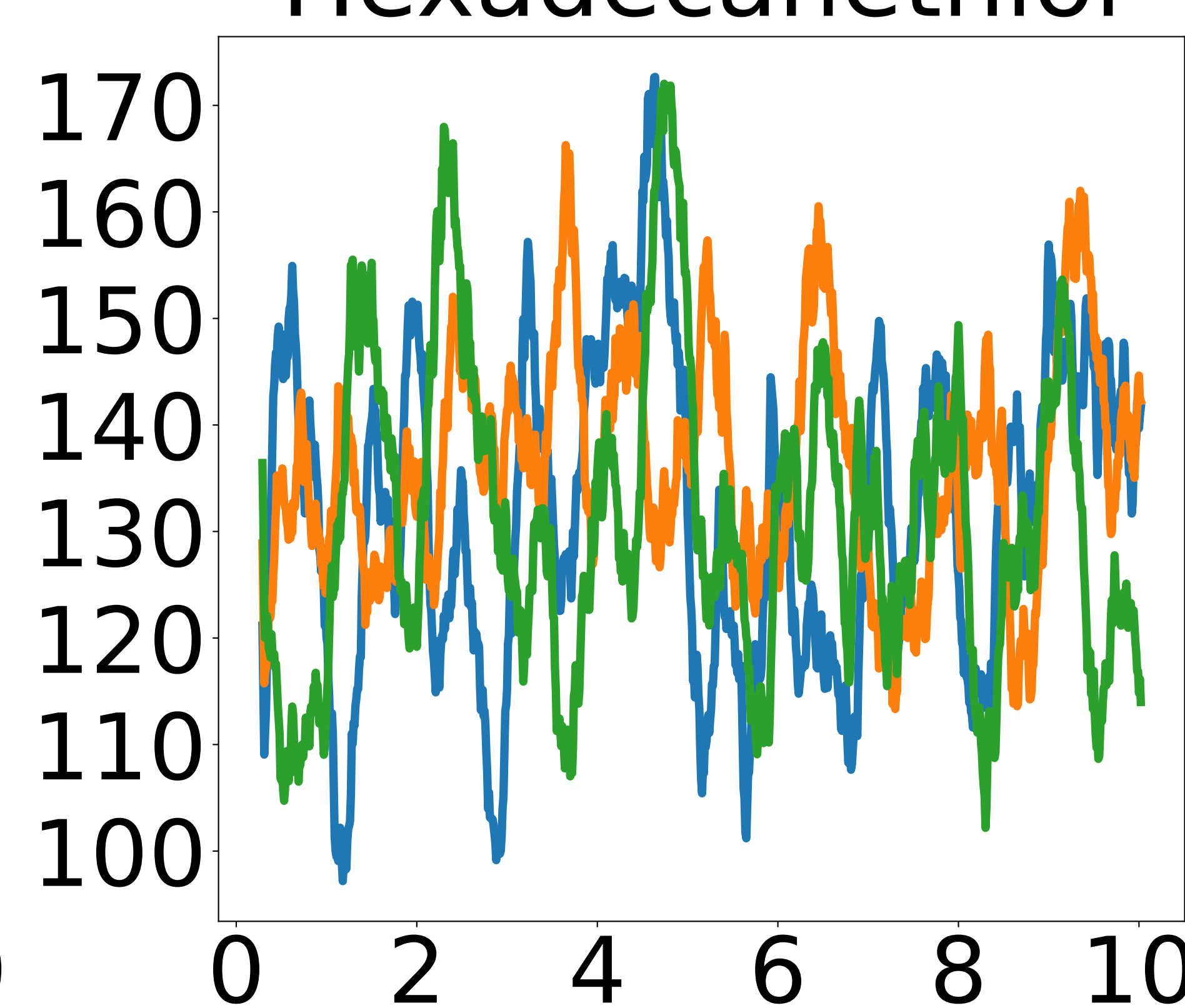
Hexadecanethiol
