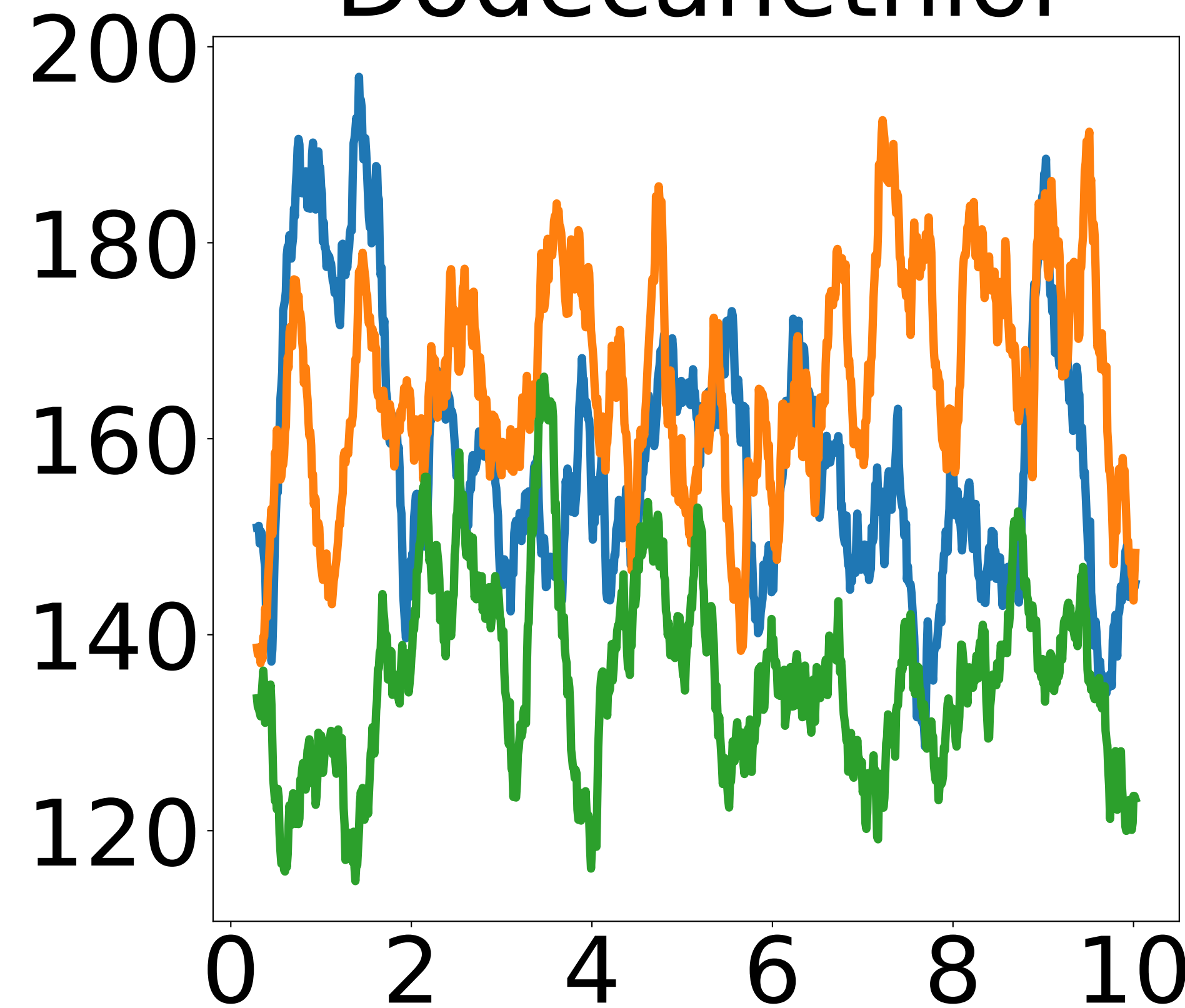
Dodecanethiol
