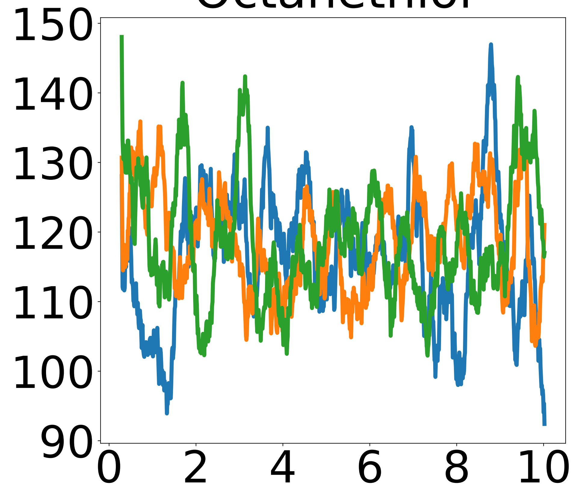
Octanethiol
