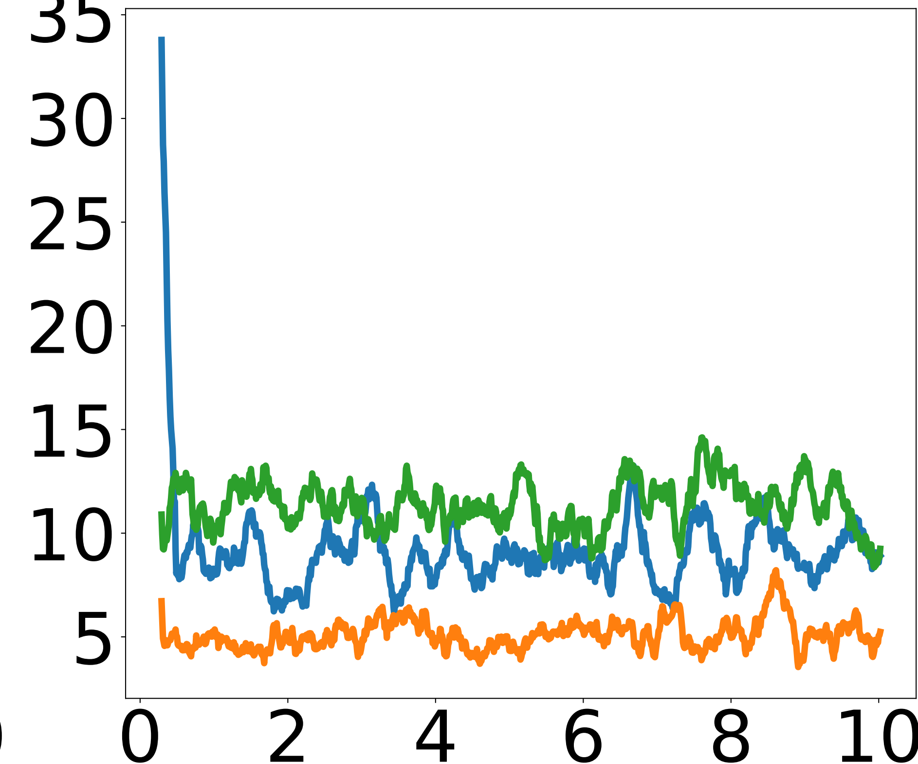
Hexadecanethiol
