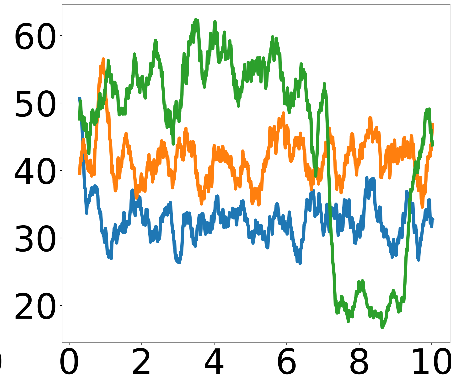
Dodecanethiol
