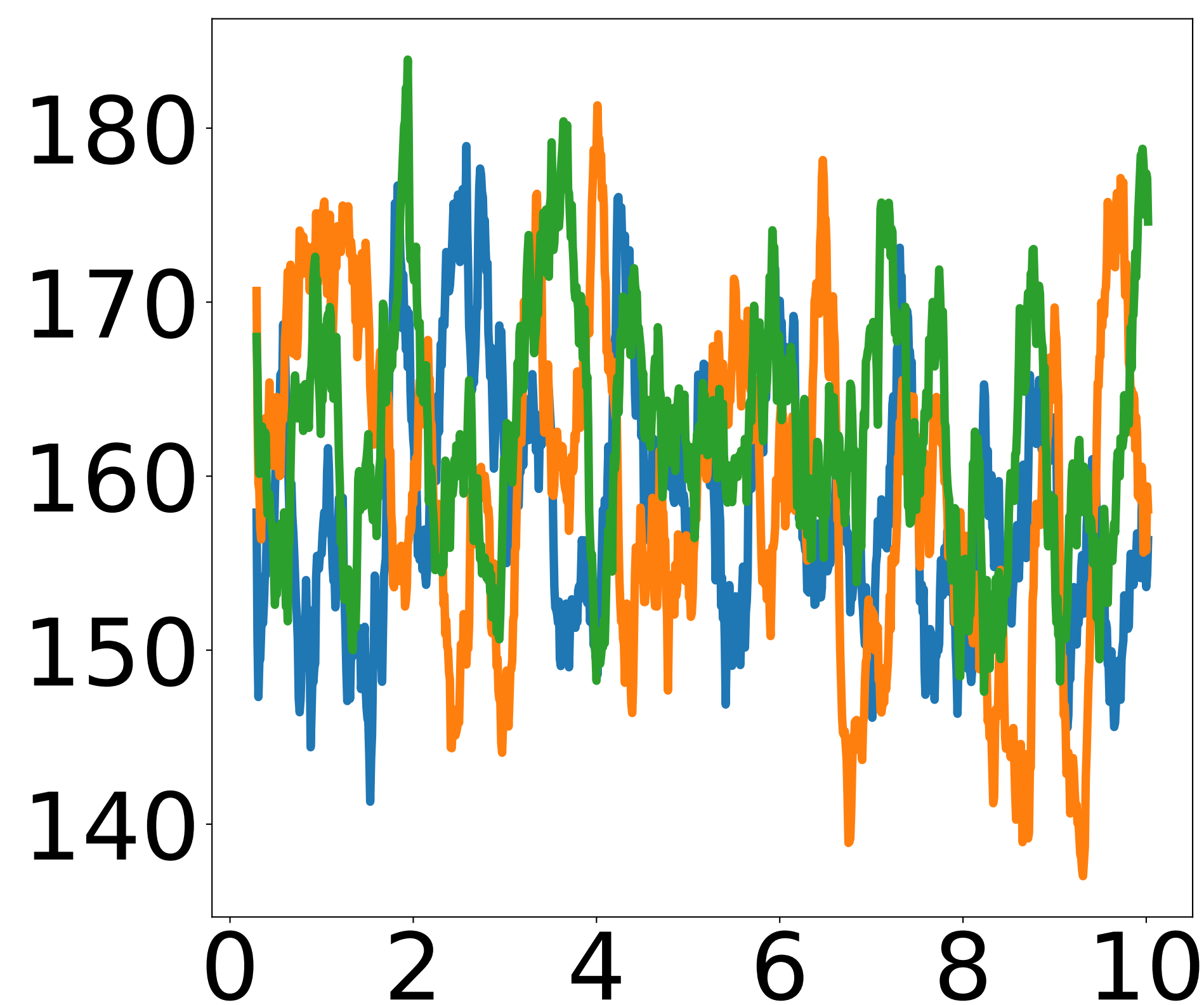
Octanethiol
