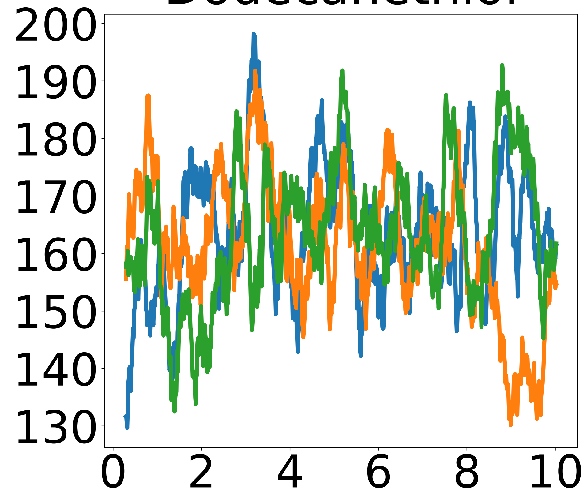
Dodecanethiol
