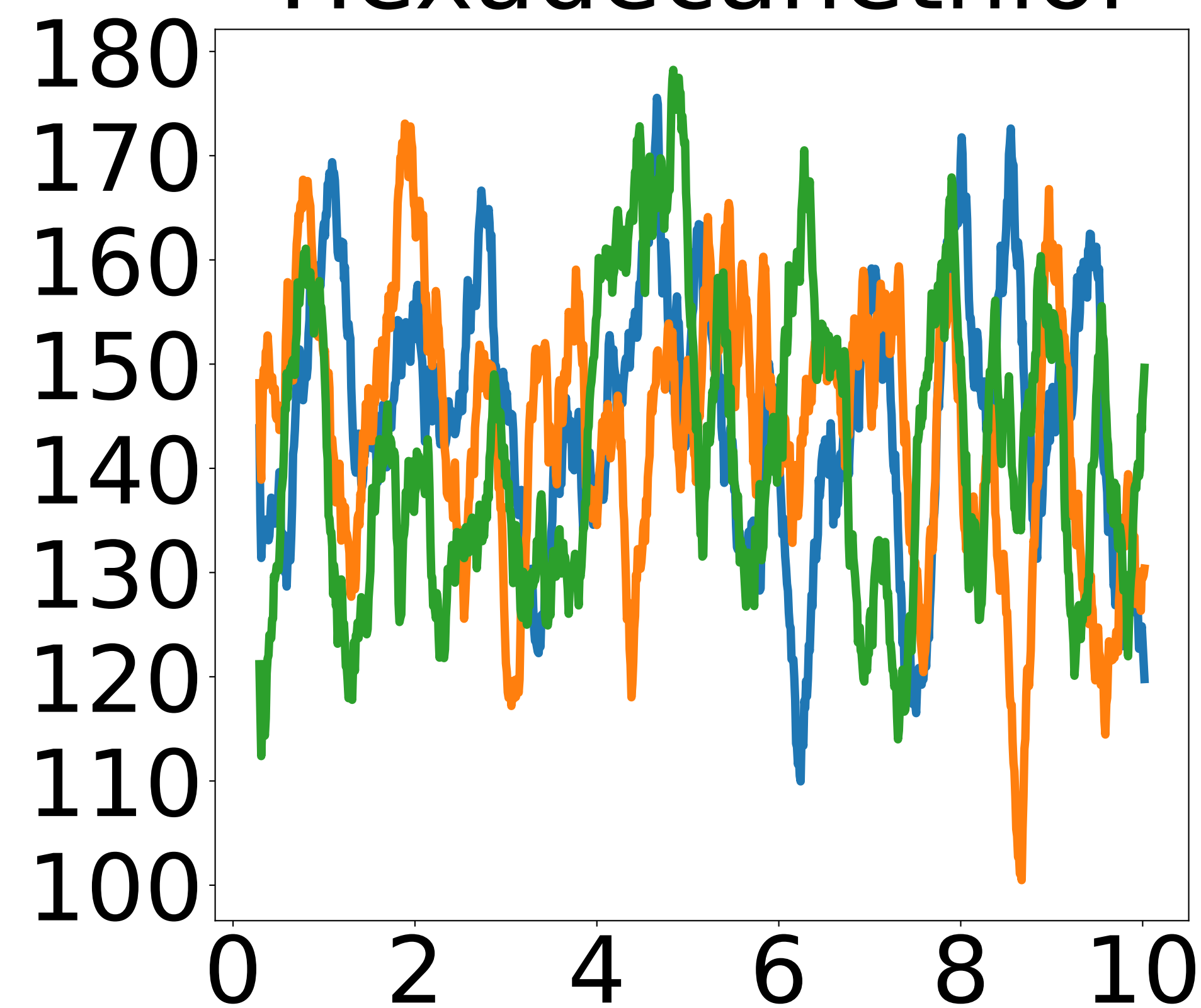
Hexadecanethiol
