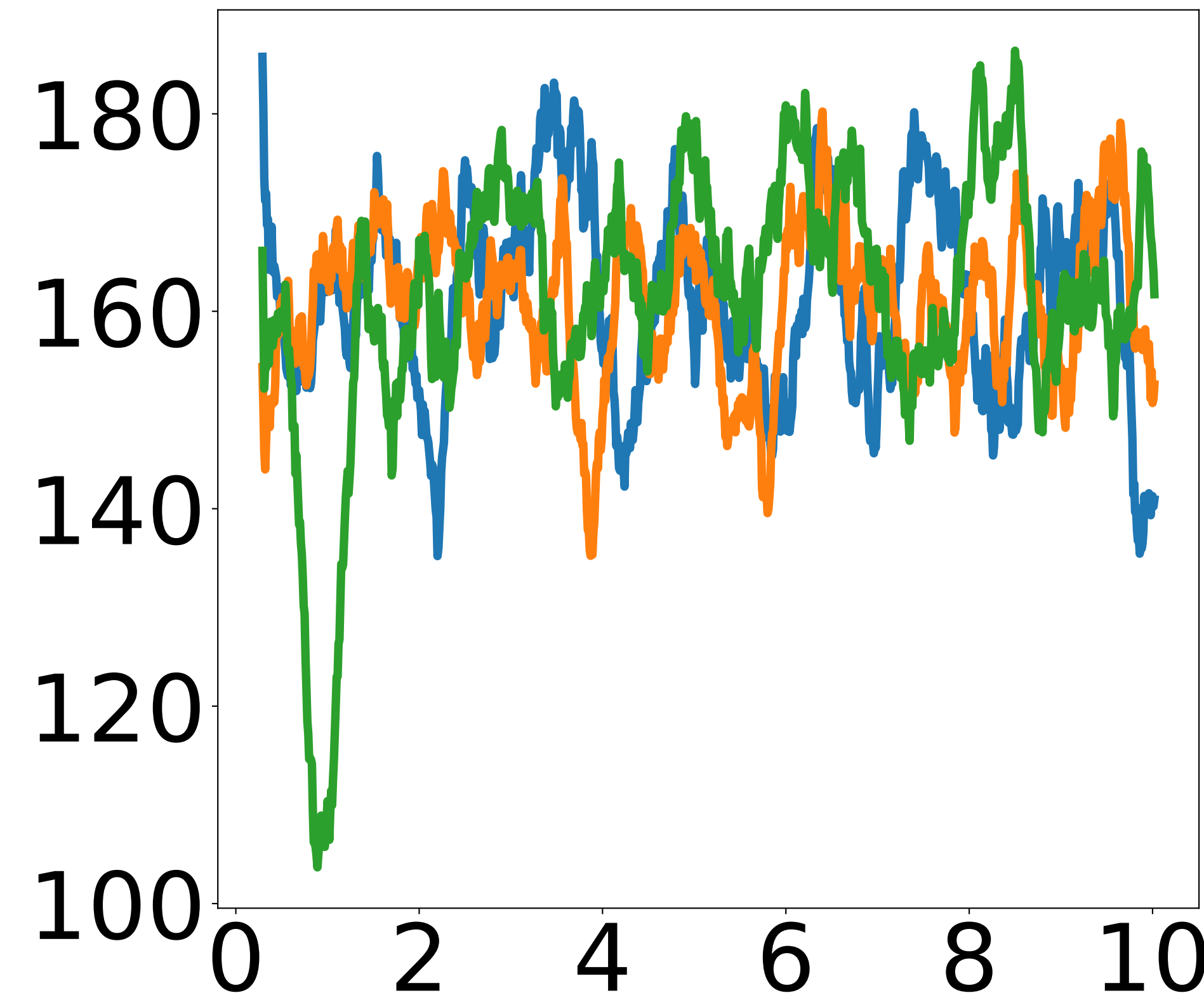
Octanethiol
