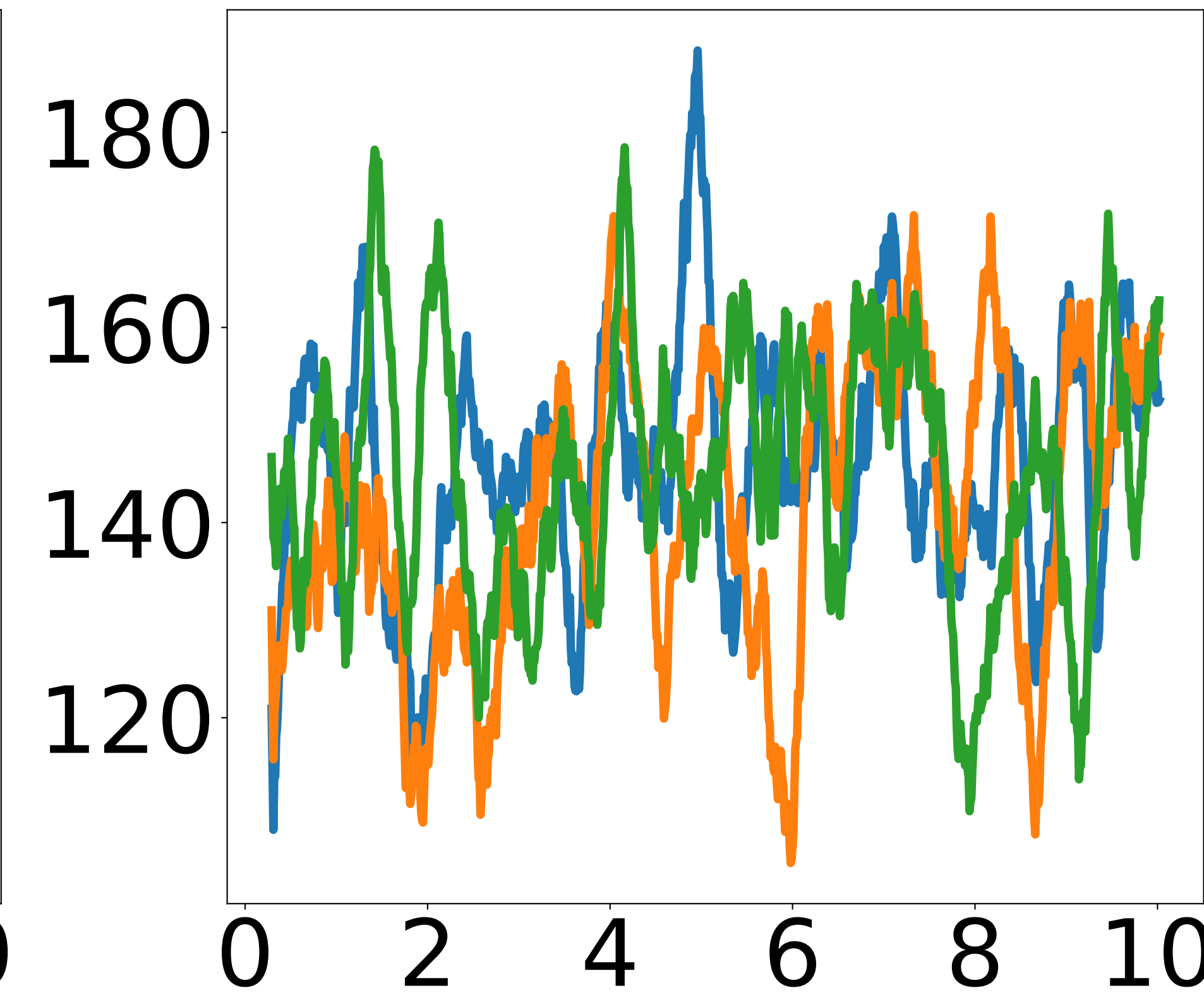
Hexadecanethiol
