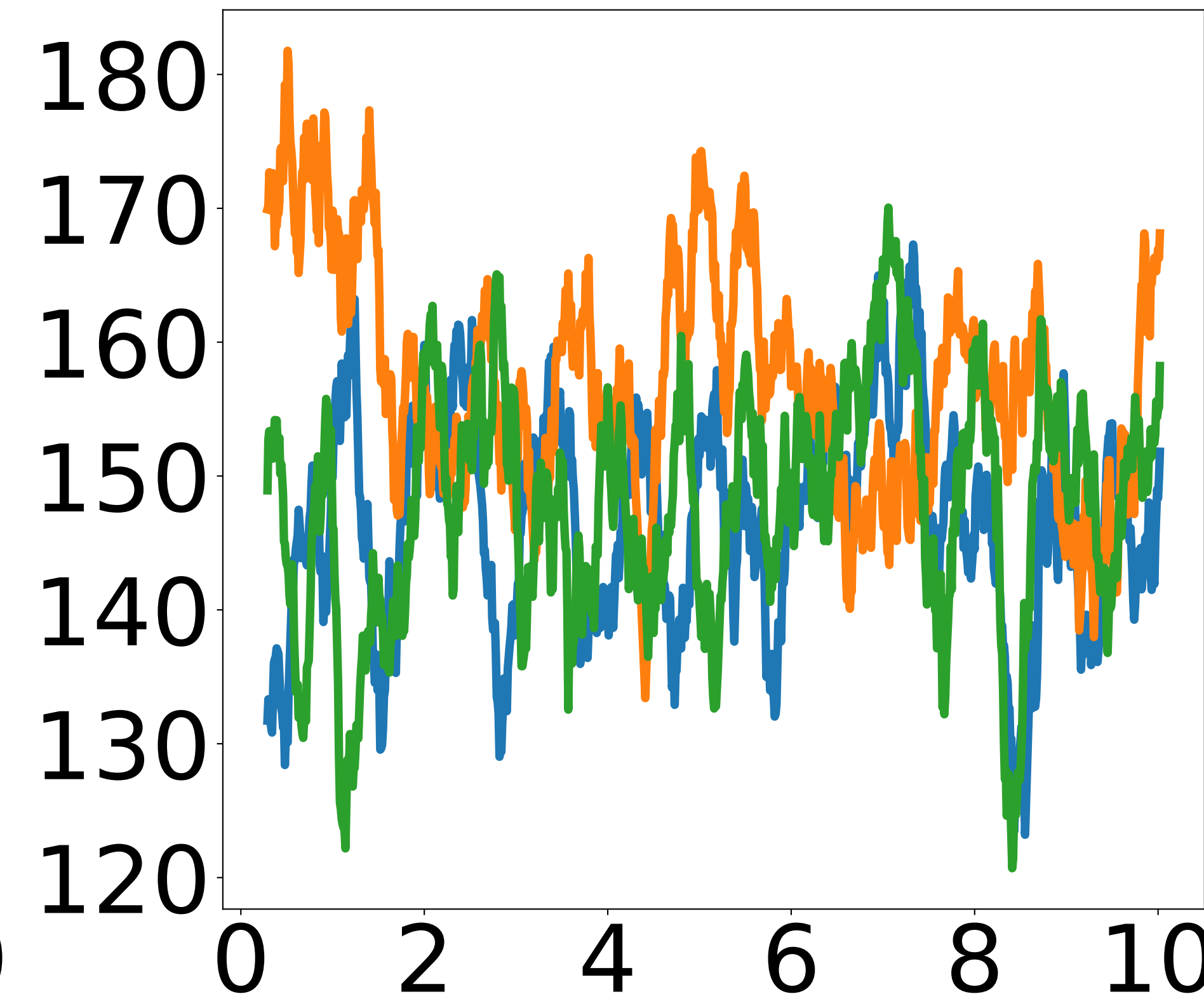
Dodecanethiol
