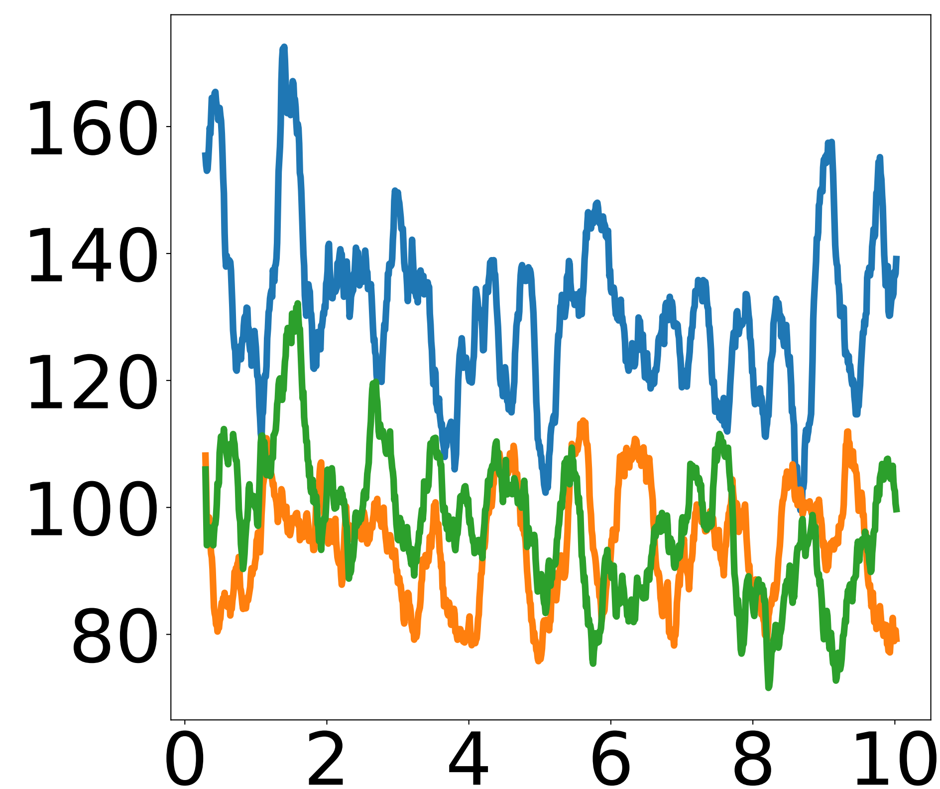
Dodecanethiol
