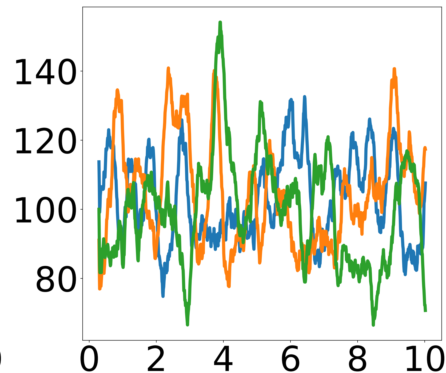
Hexadecanethiol
