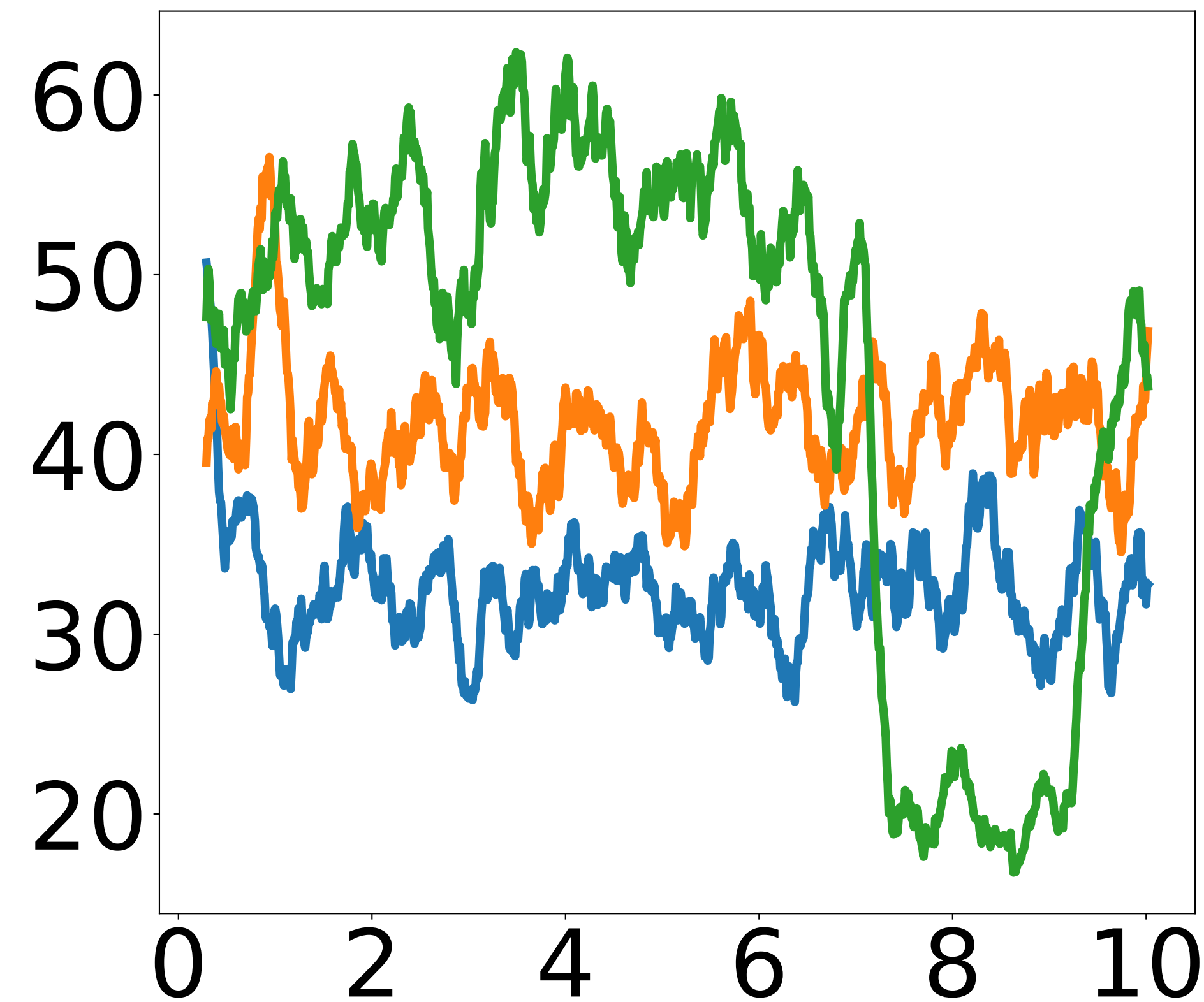
Dodecanethiol
