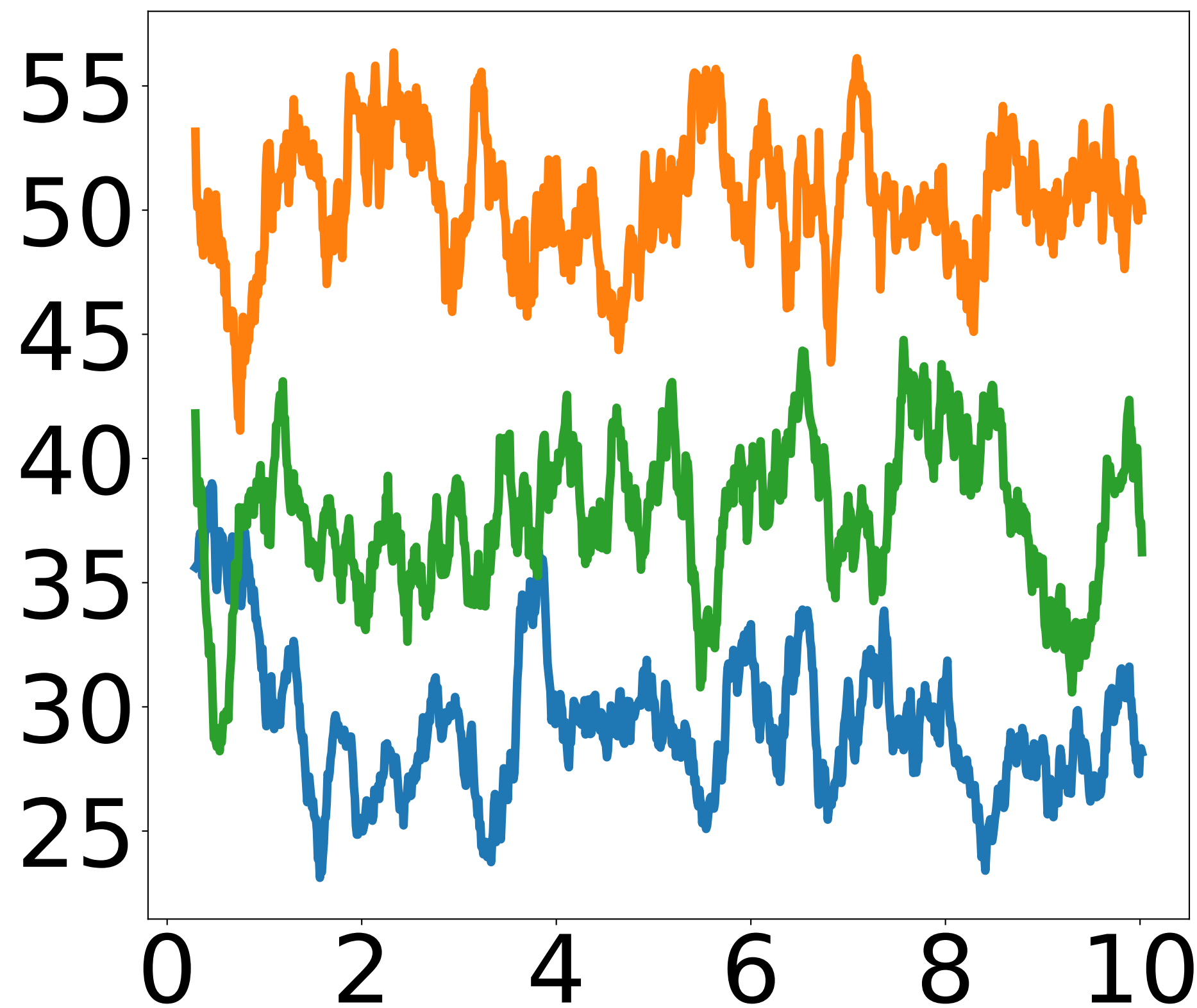
Octanethiol
