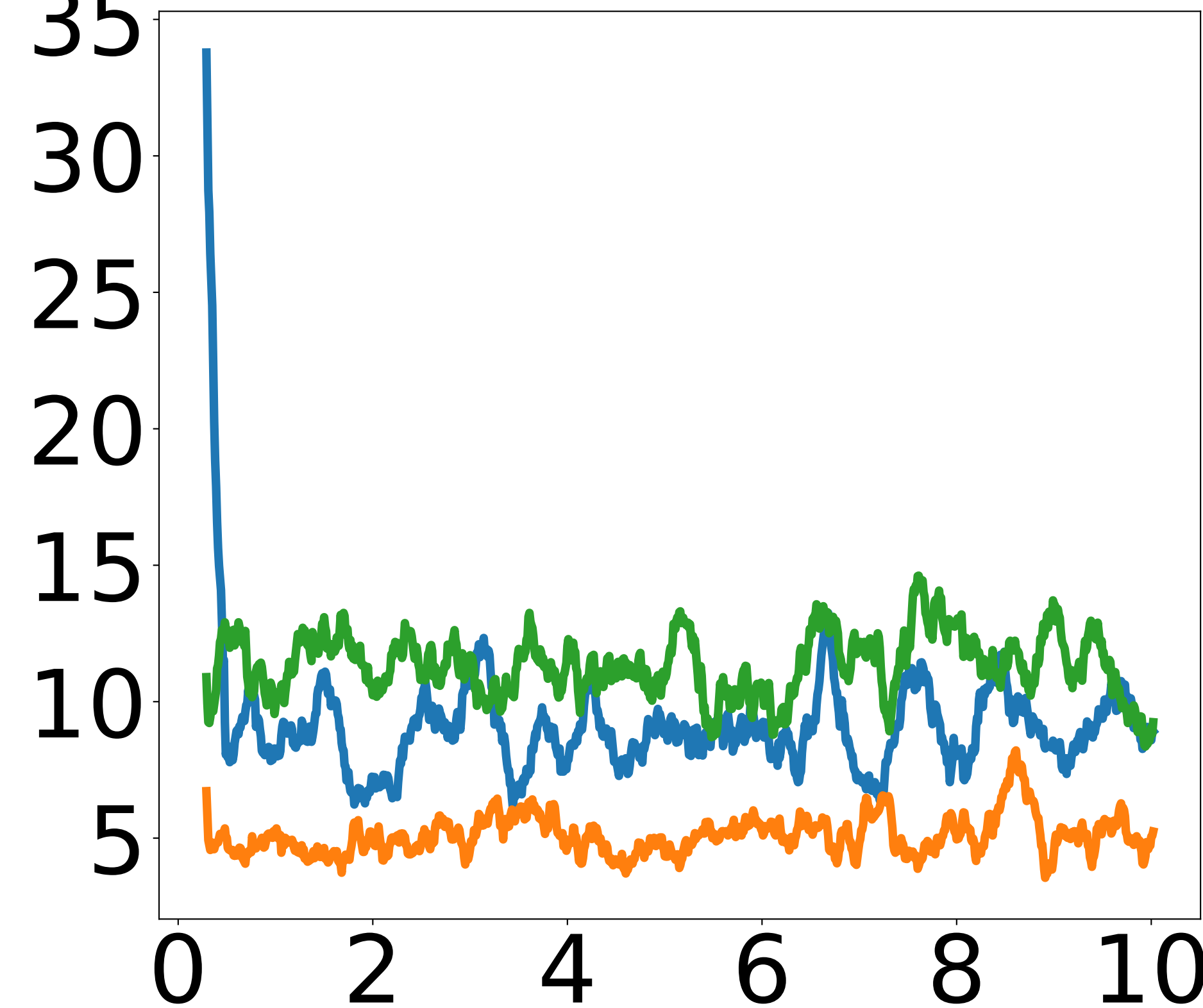
Hexadecanethiol
