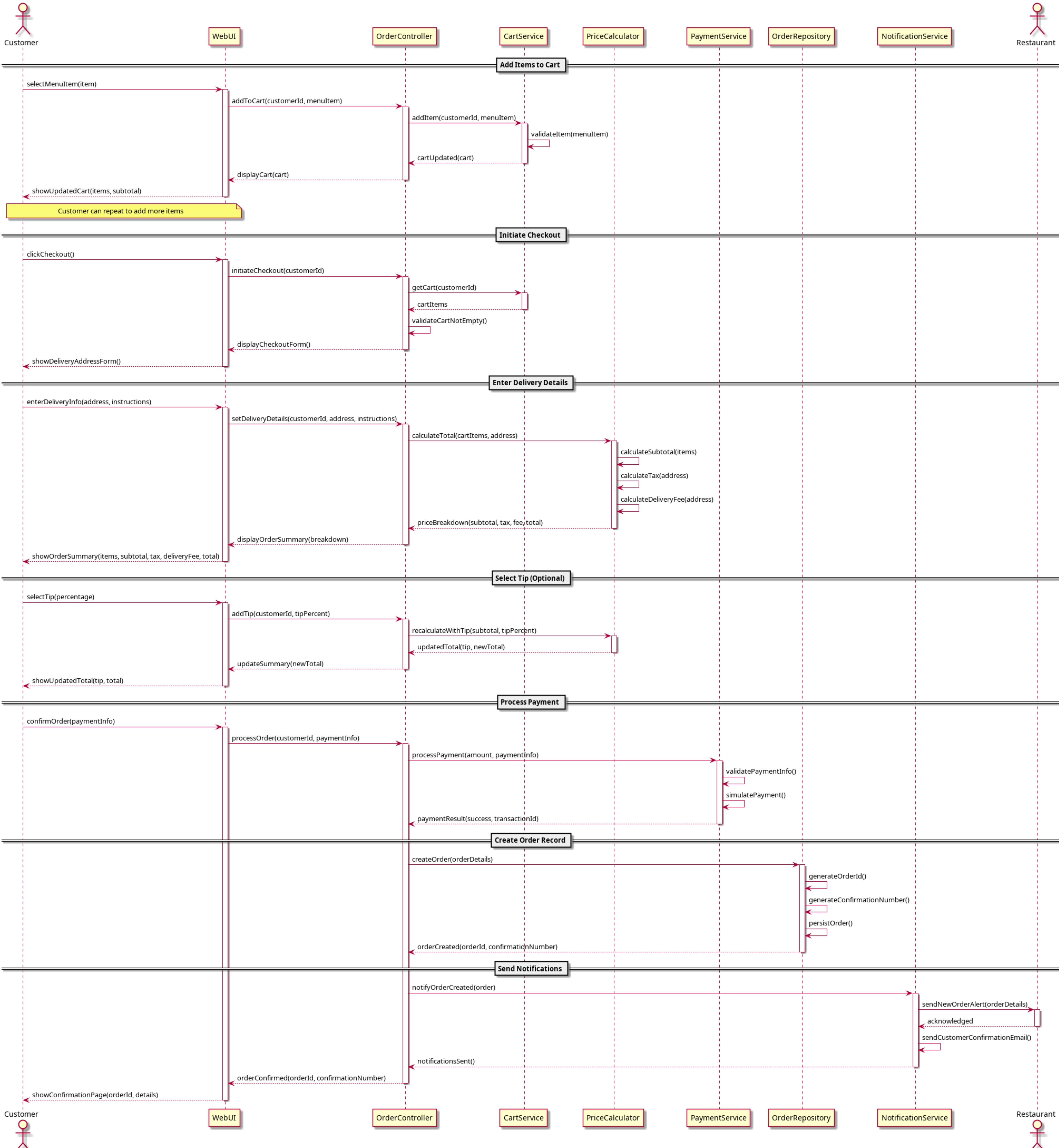
Sequence Diagram: UC6 - Create Order (Success Scenario)
