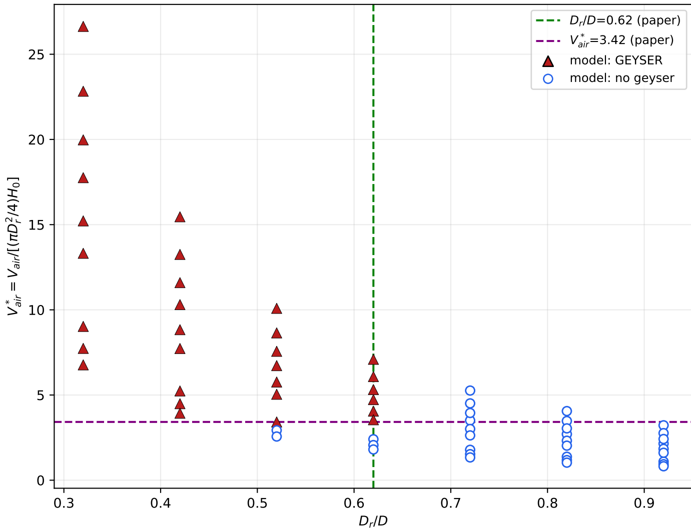
Geyser-criterion map ( D_r=16\text{-}46 mm, L_0=0.61\text{-}1.8 m, H_0=0.66\text{-}0.88 m)
