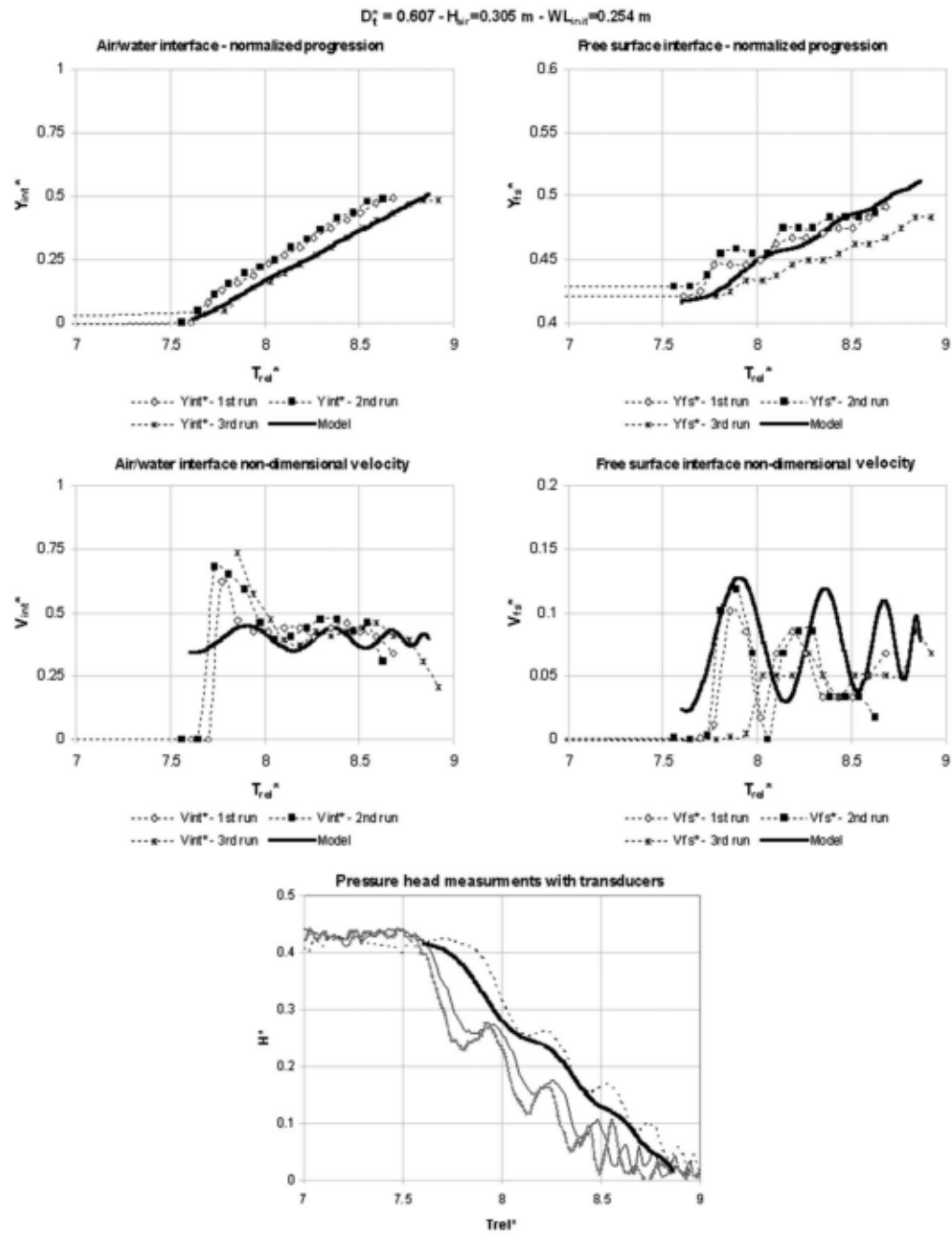
(a) Published experiment and TPA model (Vasconcelos and Wright, 2011, Fig. 10)
