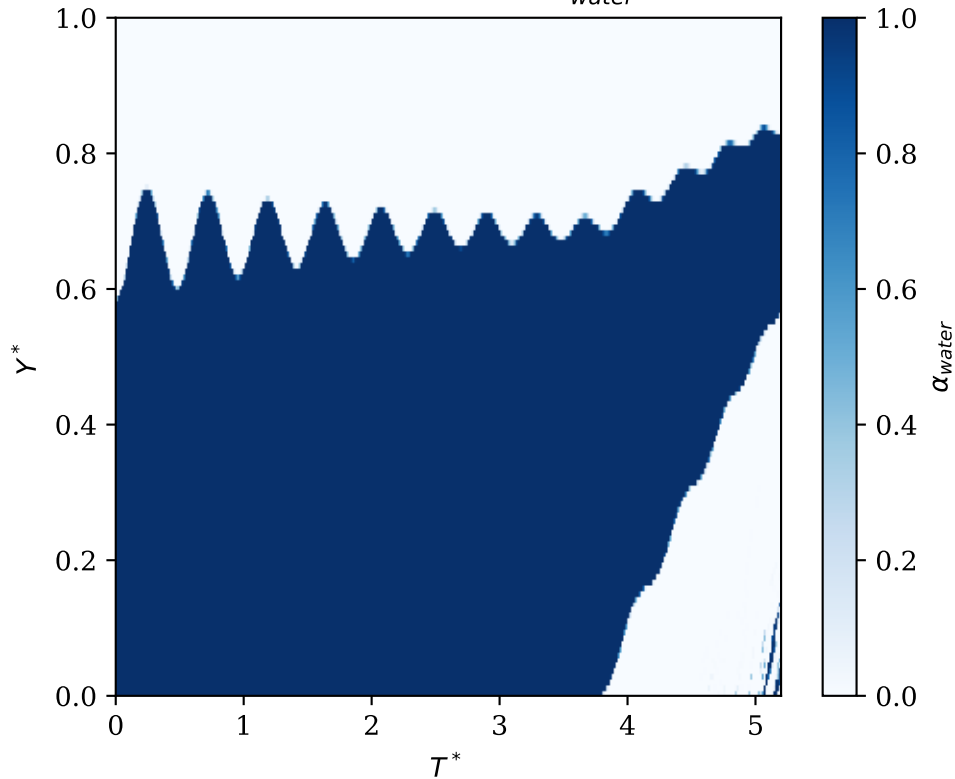
Tower centreline \alpha_{water}
