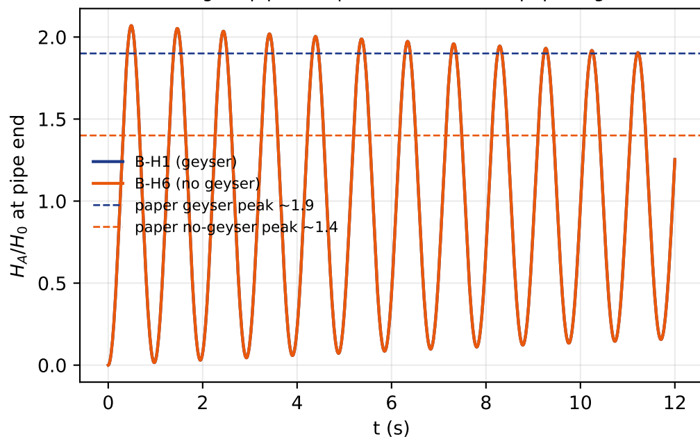
(c) Stage-1 pipe-end pressure transient (paper Fig.10)
