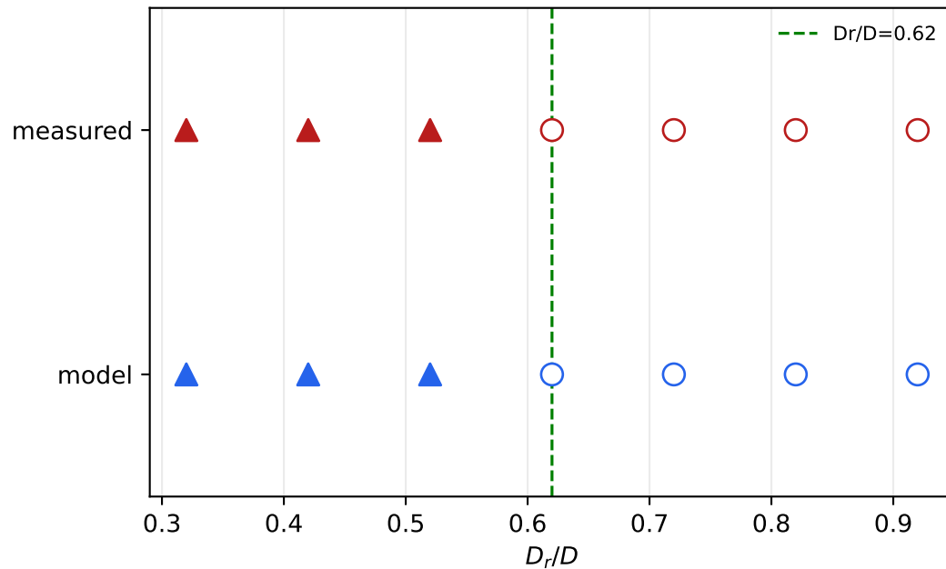
(a) Geyser (filled) vs no-geyser (open) — B-H1..B-H7
