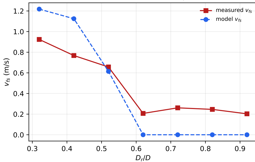
(c) Free-surface mean rise speed
