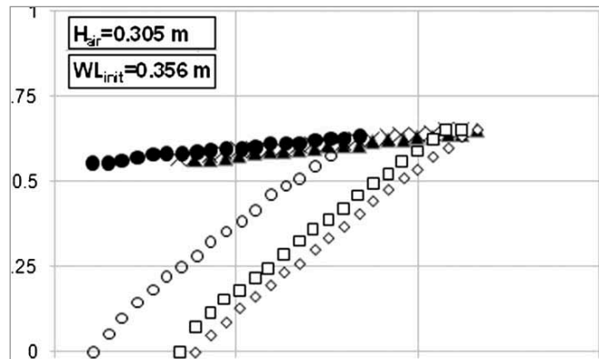
Free-surface / interface panel Vasconcelos and Wright (2011), Fig. 7
