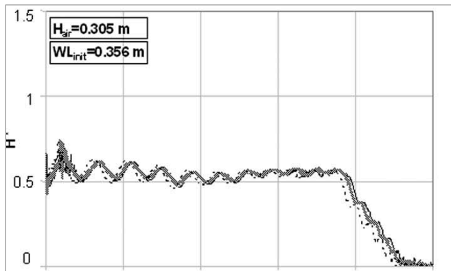
Pressure panel Vasconcelos and Wright (2011), Fig. 5
