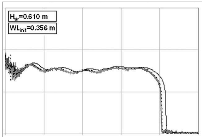
Pressure panel Vasconcelos and Wright (2011), Fig. 6
