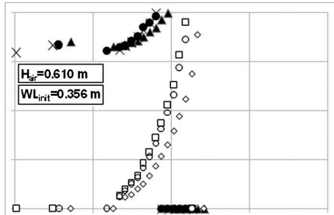
Free-surface / interface panel Vasconcelos and Wright (2011), Fig. 8
