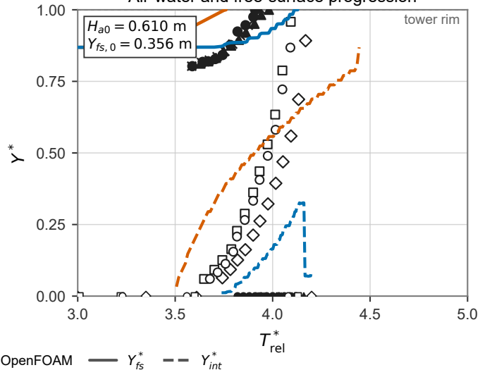
Air-water and free-surface progression
