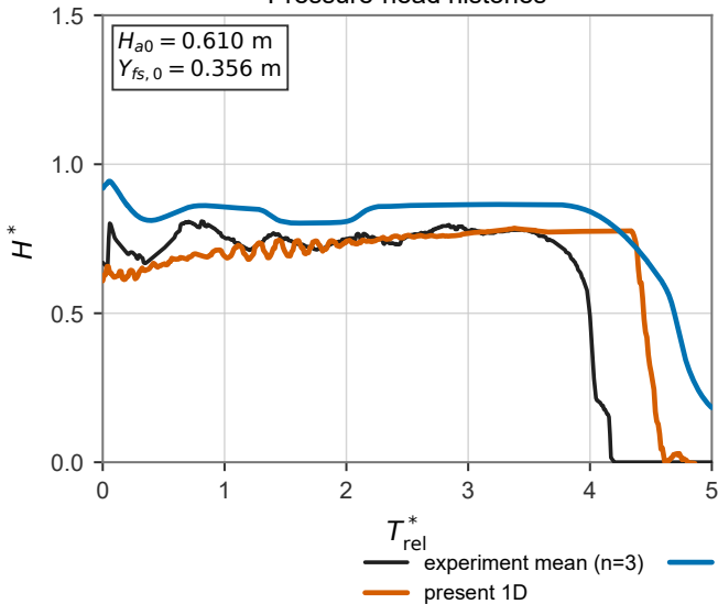
Pressure-head histories
