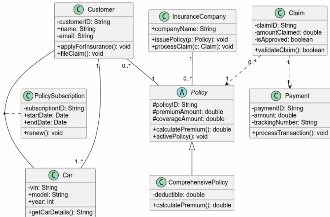
Car Insurance System - Class Diagram
