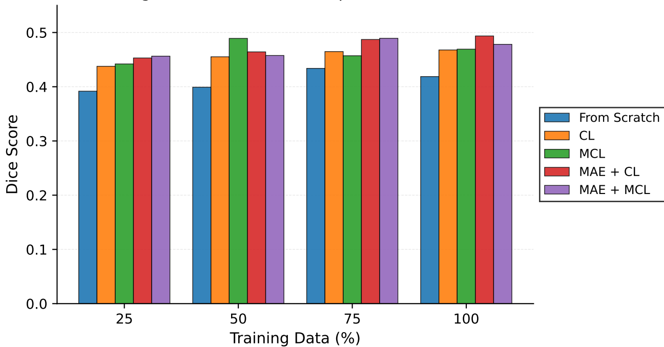
Few-Shot Segmentation: Model Comparison on ATLAS Dataset
