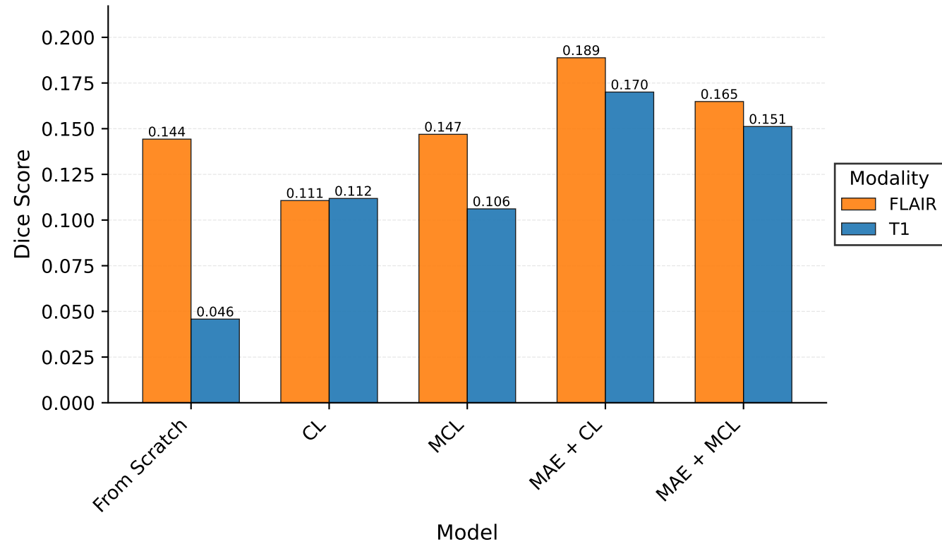
Bohn FCD: Model Performance Across Modalities
