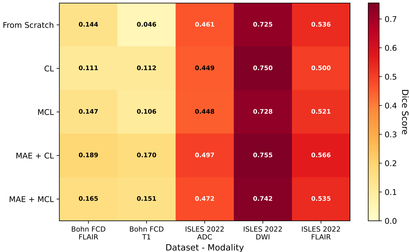
Multi-Dataset Performance Matrix: All Models and Modalities
