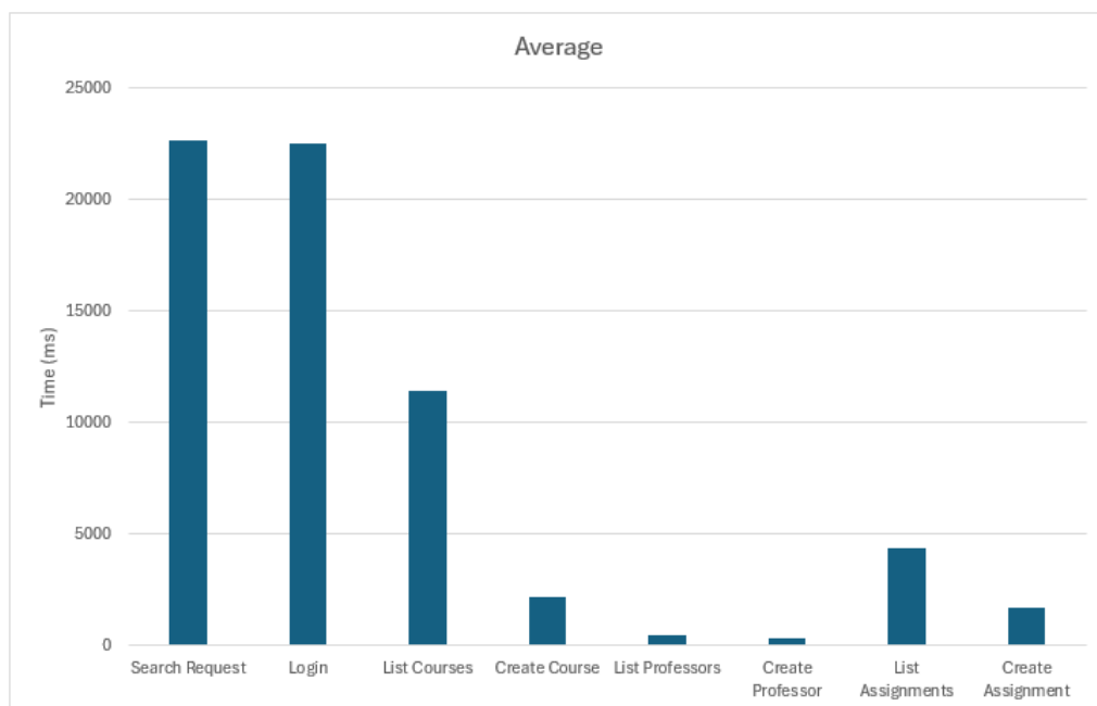
Figure 37: Average response time recorded across all tested endpoints under peak load.
