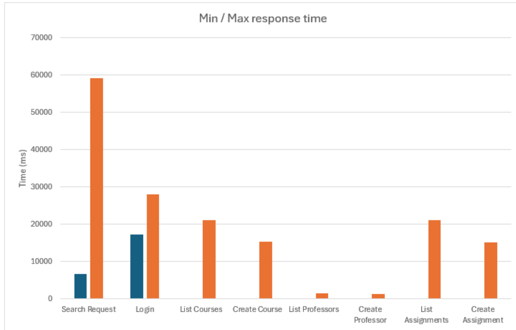
Figure 38: Minimum and maximum response times observed during the stress test.
