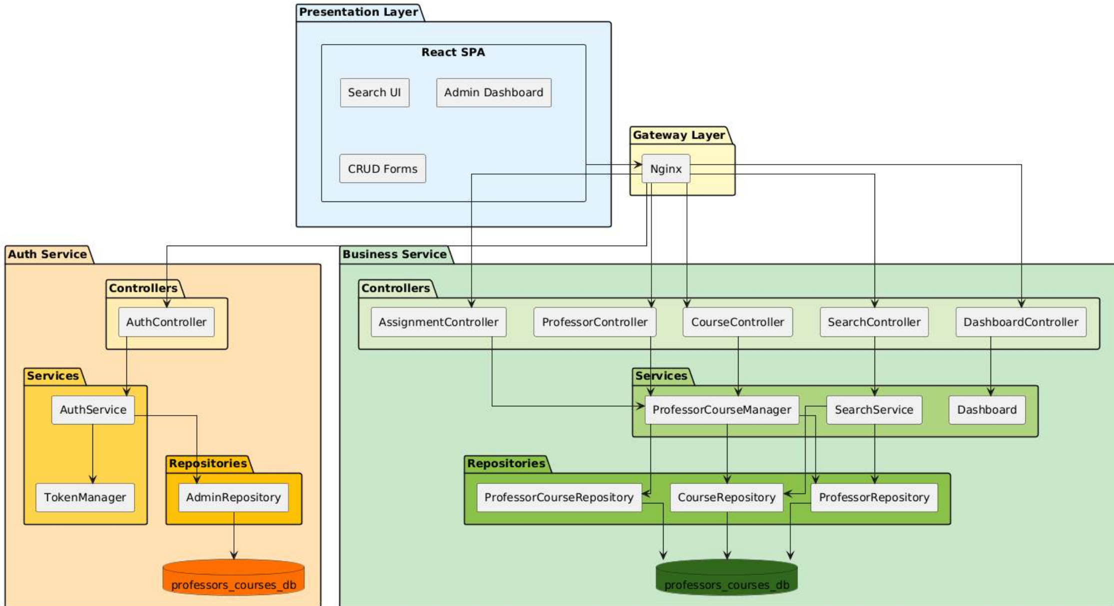
Course Finder - Architecture Diagram
