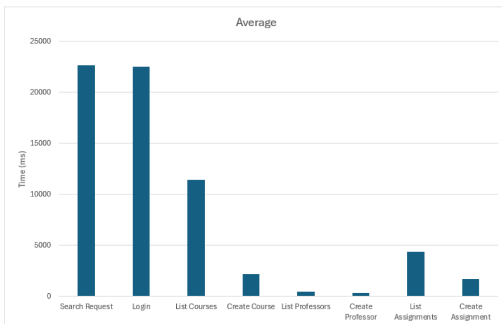
Figure 31: Average response time recorded across all tested endpoints under peak load.
