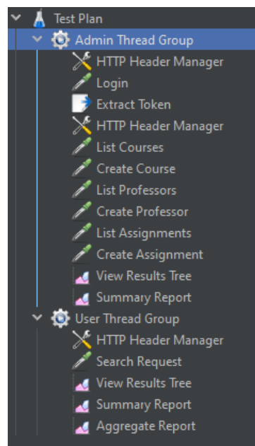
Figure 30: JMeter test plan structure showing the two Thread Groups used for administrator workflows and high-load search endpoint stress testing.
