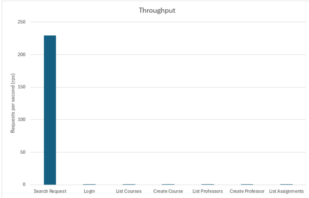
Figure 33: Throughput measured during the execution of the stress test.
