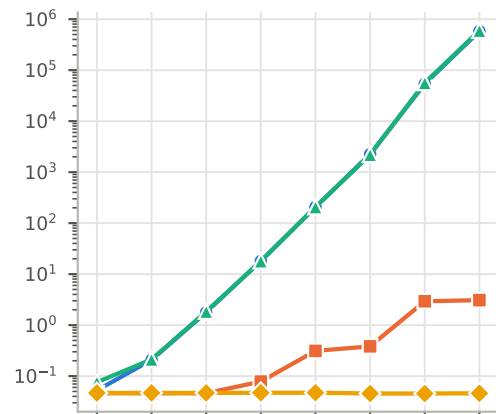
Erase
