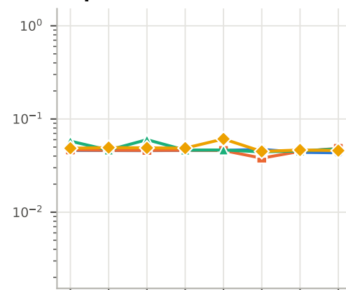
AddBefore
