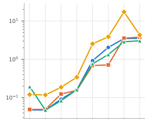
Size
