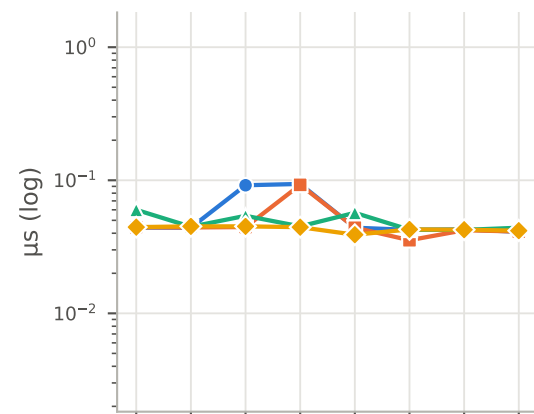
Find
