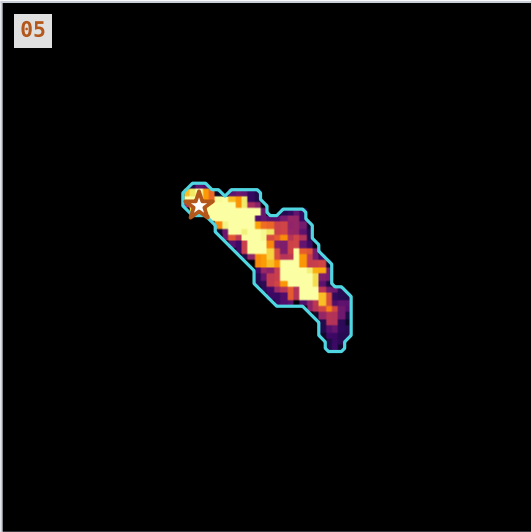
Connected-component mask
