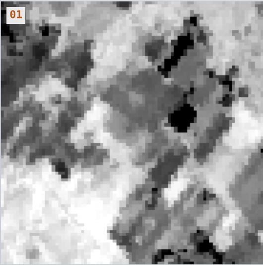
L1 radiance
