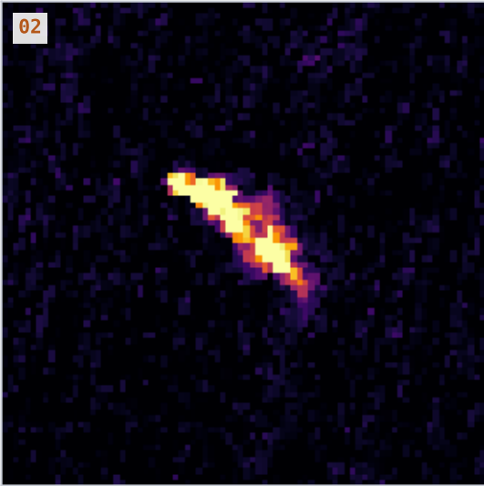
Matched filter
