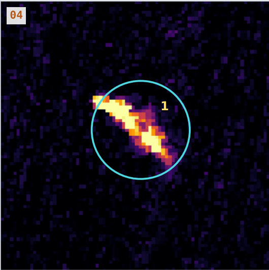
2σ candidates
