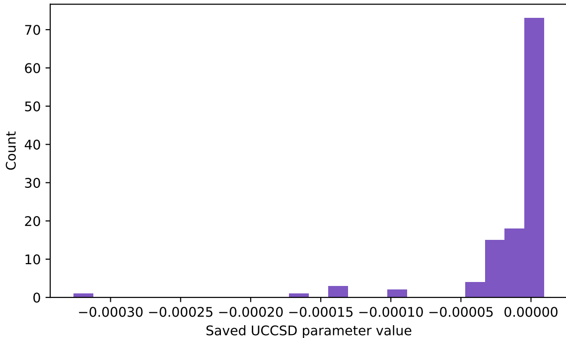
Distribution of 117 saved UCCSD parameters
