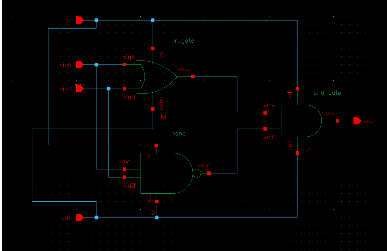
Schematic
