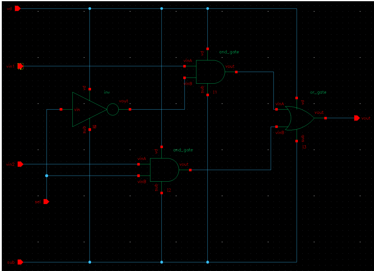
Schematic
