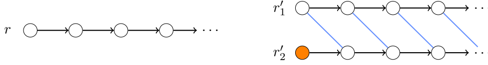
Figure 5.2: \mathfrak{J}_1 (Left) and \mathfrak{J}'_1 (Right)
