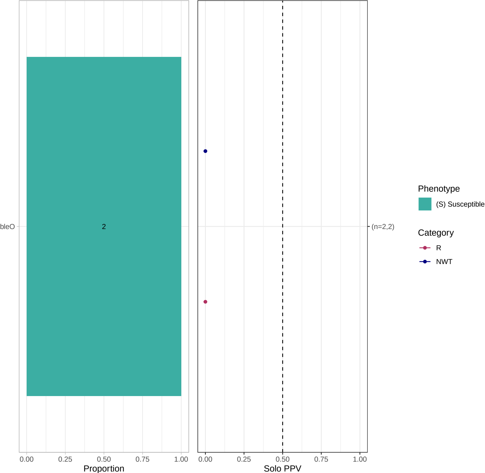
Solo markers for class: Glycopeptides, Glycopeptide, GLYCOPEPTIDE, vancomycin, VANCOMYCIN vs phenotype for drug: VAN
